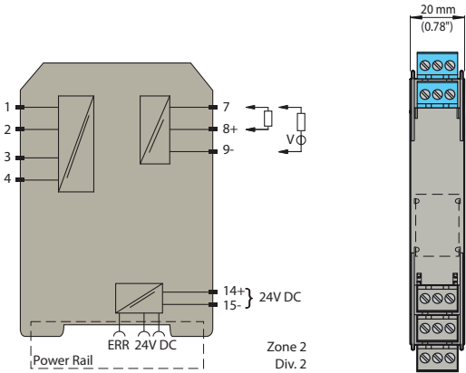
Wiring Diagram
