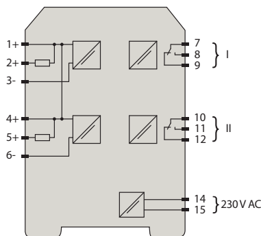
Wiring Diagram
