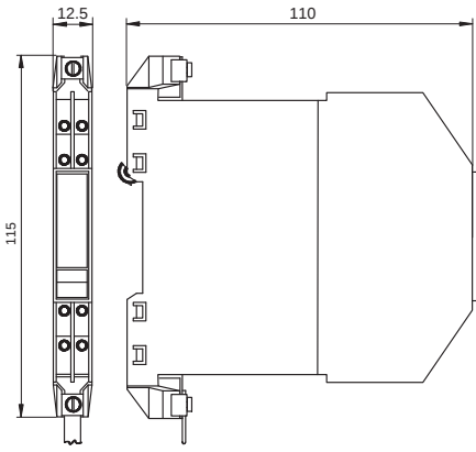
Approximate Dimensions
