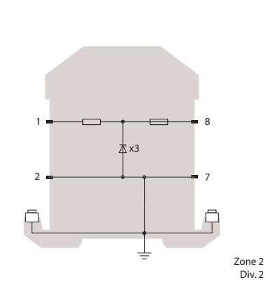
Wiring Diagram
