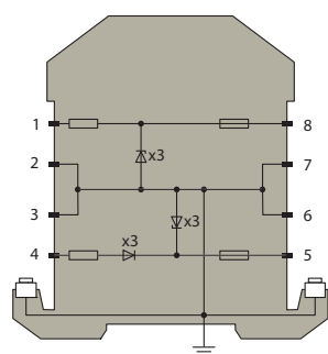
Wiring Diagram
