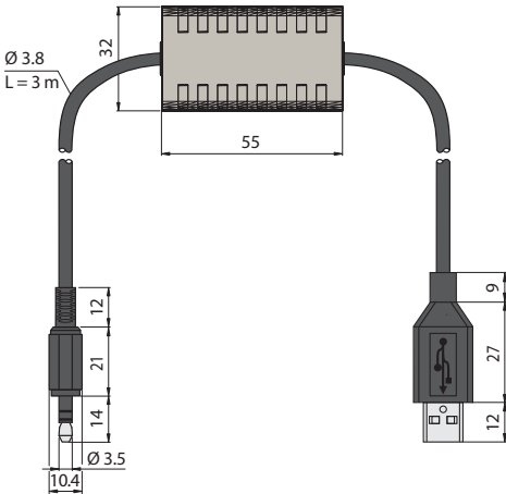
Approximate Dimensions
