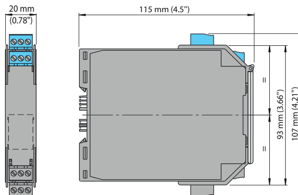
Approximate Dimensions
