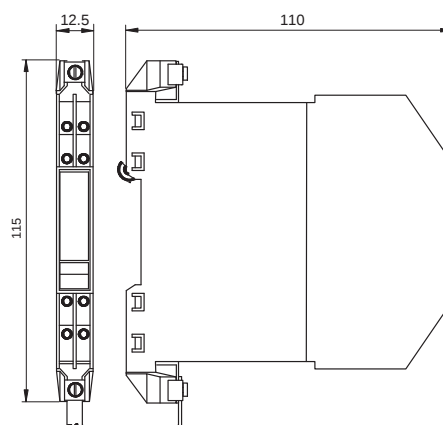
Approximate Dimensions
