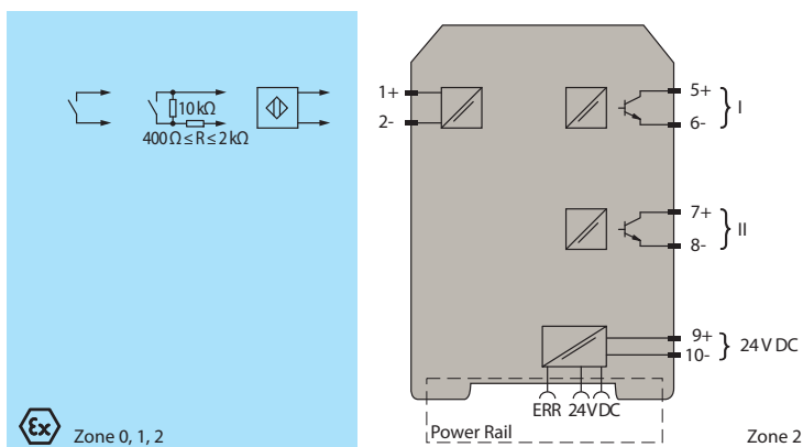
Wiring Diagram
