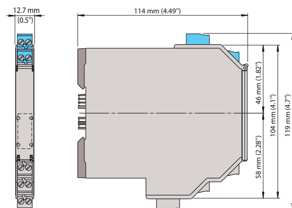
Approximate Dimensions
