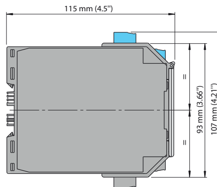
Approximate Dimensions
