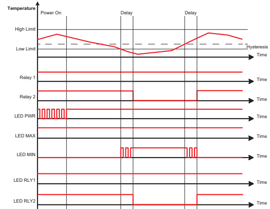
Under-temperature alarm (U)
