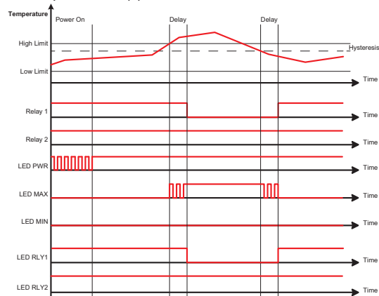
Over-temperature alarm (O)
