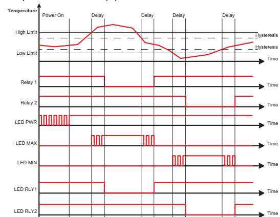
Temperature window alarm (W)
