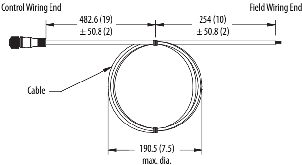
Cable Coiling
