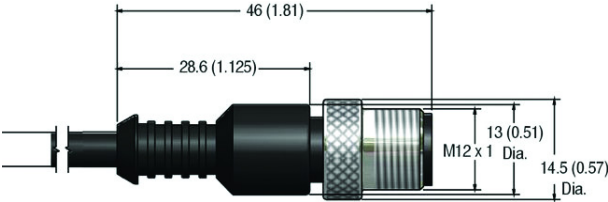
M12 Connector End of Patchcord
