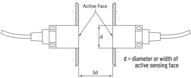
Figure 25 - Spacing Between Opposing Sensors
