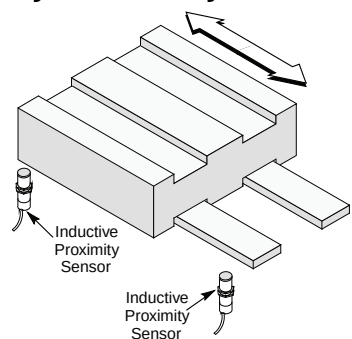
Figure 42 - Grinding Machines
