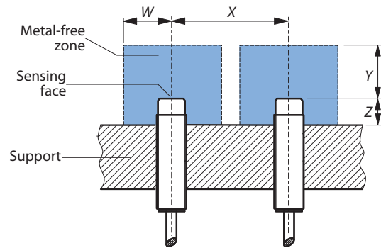
Figure 38 - Unshielded Sensors
