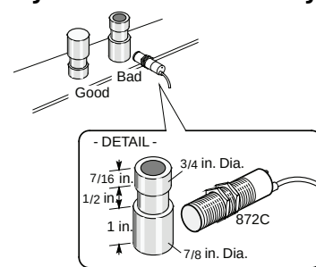
Figure 51 - Railroad Yard Position Sensing
