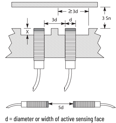
Figure 18 - Tubular-style Long-range Sensing (872C)
