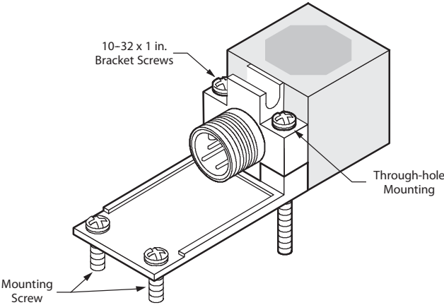
Figure 12 – Typical Application
