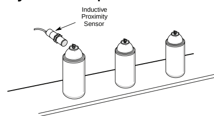
Figure 48 - Food Industry
