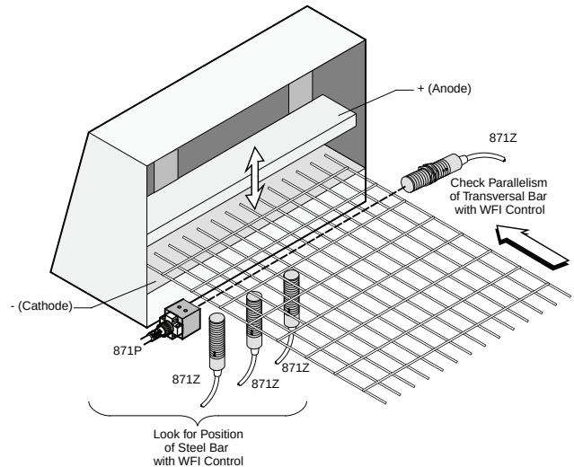
Figure 58 - Elevator Positioning
