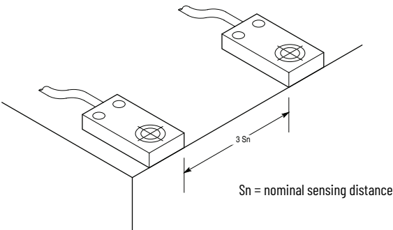
Figure 22 - Miniature Flat Pack Style (871FM)
