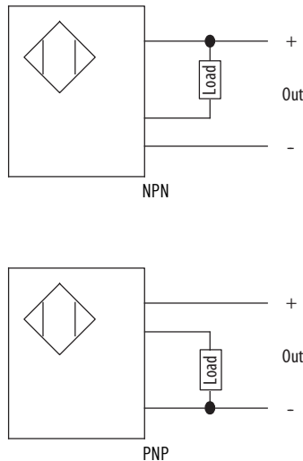
Figure 3 - NPN and PNP
