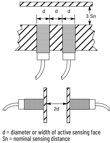
Figure 16 - Tubular Style
