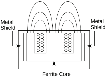
Figure 14 - Shielded Sensor
