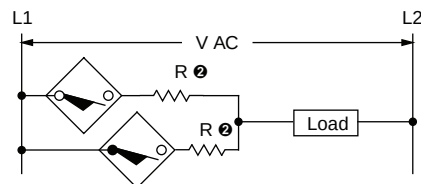
Figure 13 - Wiring Diagram for Parallel Connected AC Sensors
