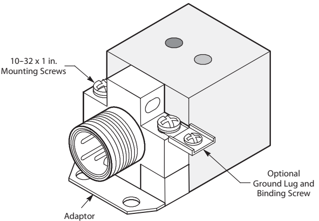
Figure 11 - Typical Application
