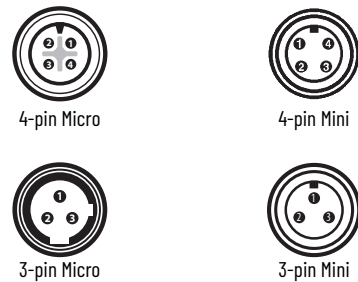
Figure 5 - Connectors
