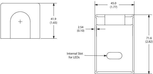
Figure 14 – Catalog Number 871A-KCT40-T
