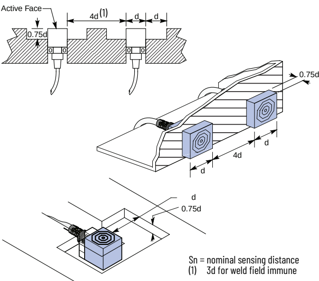
Figure 34 - 871P VersaCube – 4-Wire
