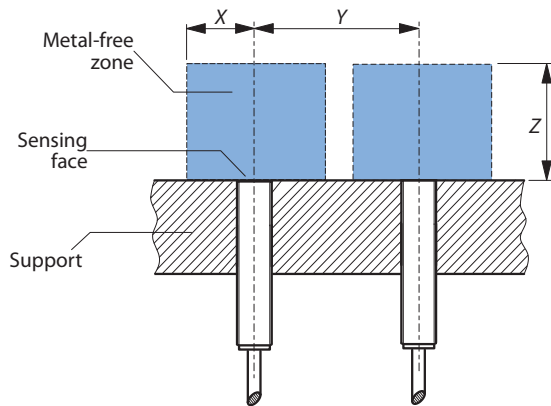
Figure 37 - Shielded Sensors
