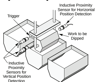
Figure 41 - Plating Line
