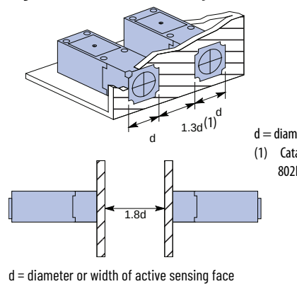
Figure 20 - Limit Switch Style (802PR)
