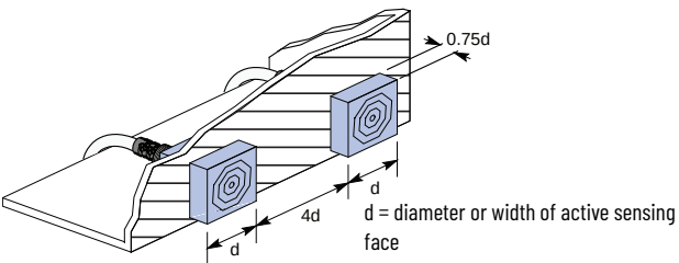
Figure 36 - Spacing Between Opposing Sensors
