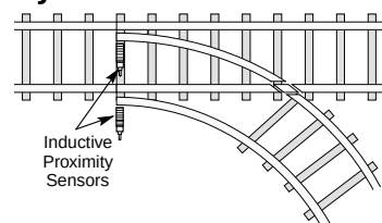
Figure 51 - Railroad Yard Position Sensing
