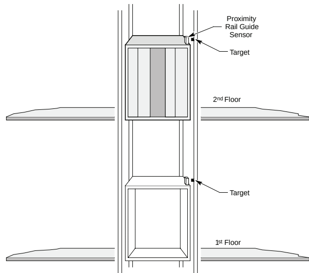
Figure 58 - Elevator Positioning
