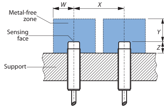
Figure 38 - Unshielded Sensors
