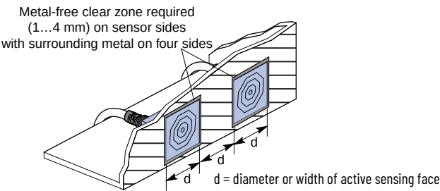
Figure 24 - 871P VersaCube – 4-Wire
