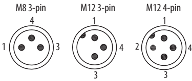
Figure 61 - 8 mm, 12 mm, 18 mm, and 30 mm Pinouts
