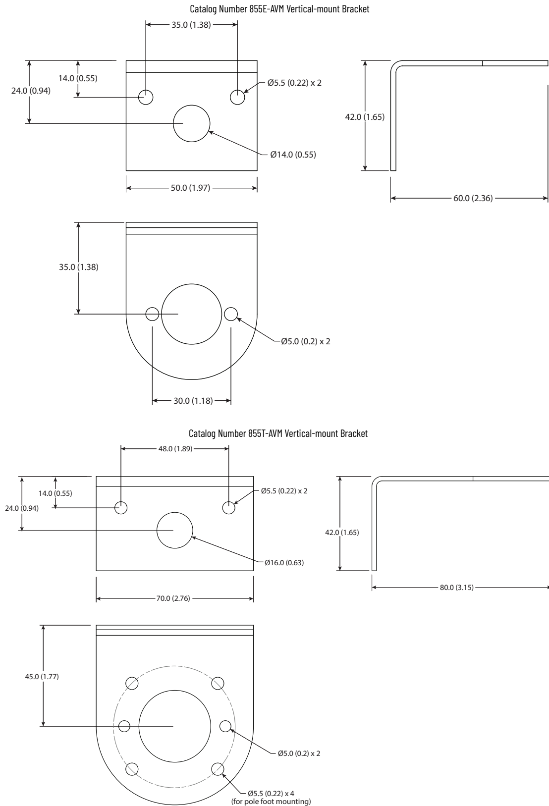
Figure 12 - Component and Accessory Dimensions
