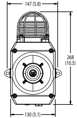
855HM-C Metal Horn with LED Beacon
