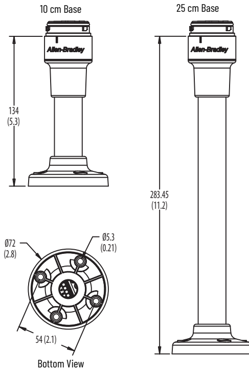
Flange-style Base with M12 Micro Connector (Male)
