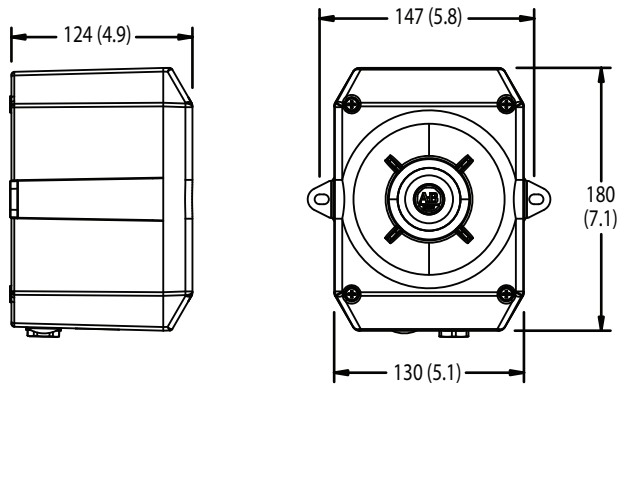
855HM Metal Horn
