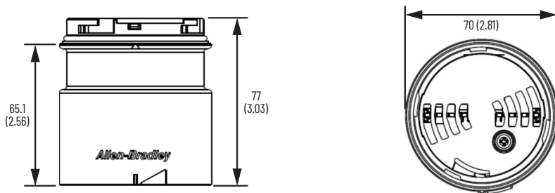
Figure 16 - Component and Accessory Dimensions
