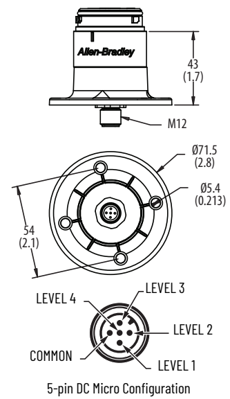
Flange-style Base with M12 Micro Connector (Male)
