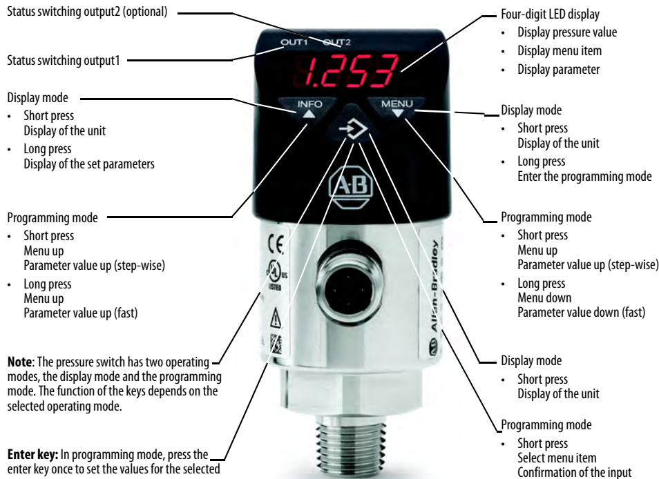
Figure 2 - Keys and Functions
