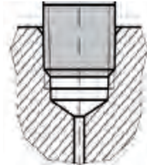
Tapered Thread (NPT)
