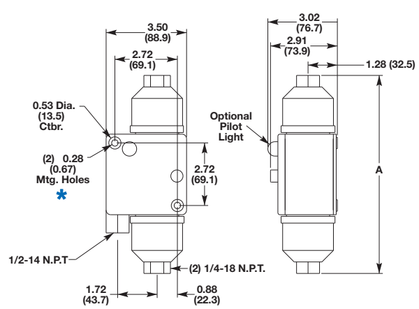
Figure 61 - Type 4 & 13 Pressure Difference Control Operator
