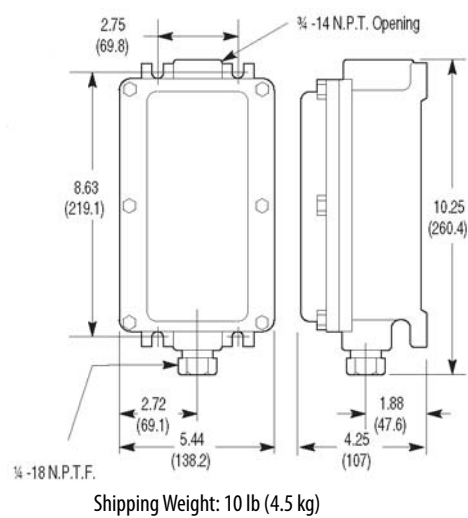
Figure 27 - Type 4X
