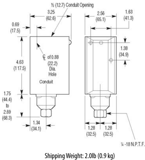
Figure 26 - Type 4 & 13
