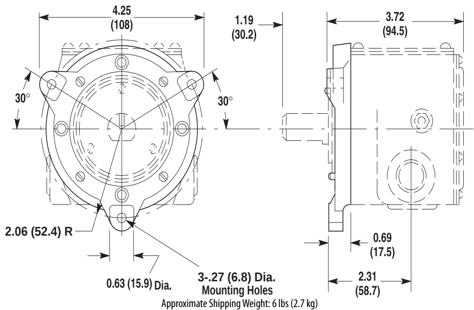
Figure 94 - Flange Mounting (Three-Point) Arrangement Type (Cat. Nos. 808-J2_, -K2_, -M2_, -R2_)
