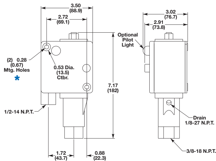
Figure 62 - Type 4 & 13 (Piston)
