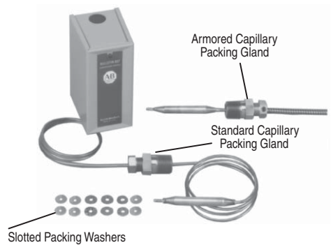
Figure 71 - Packing Glands
