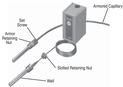
Figure 70 - Thermostat Wells
