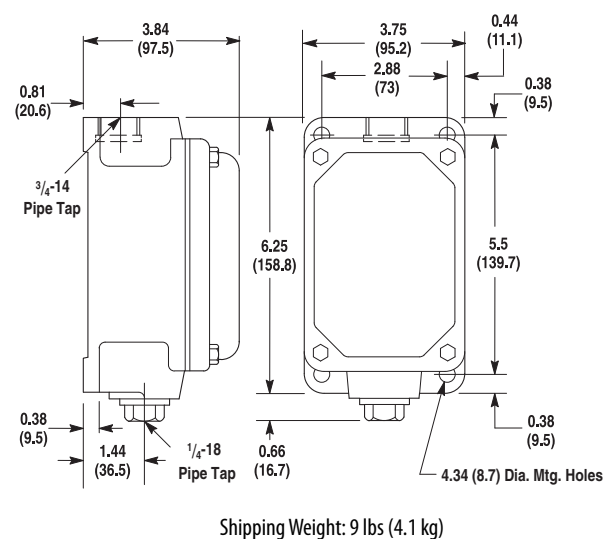
Figure 20 - Type 7 & 9 and 4 & 13
