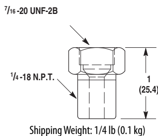
Figure 21 - Cat. No. 836-N1
