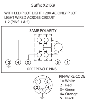
Figure 55 - With Pilot Light (2)
