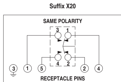
Figure 55 - With Pilot Light (2)
