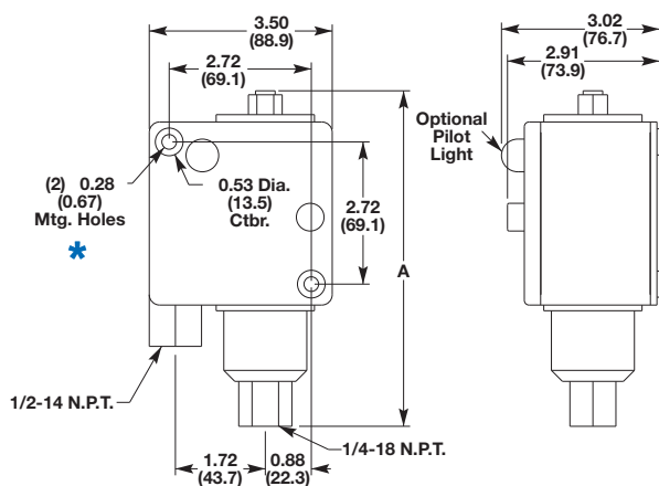
Figure 60 - Type 4 & 13 (Bellows)
