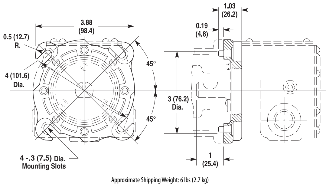
Figure 95 - Flange Mounting (Four-Point) Arrangement Type (Cat. Nos. 808-J3_, -K3_, -M3_, -R3_)
