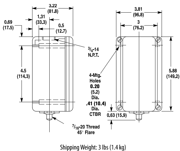
Figure 19 - Type 4 & 13
