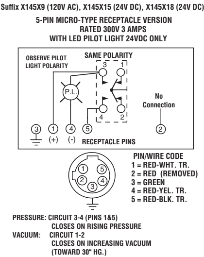
Figure 59 - With Pilot Light (2)
