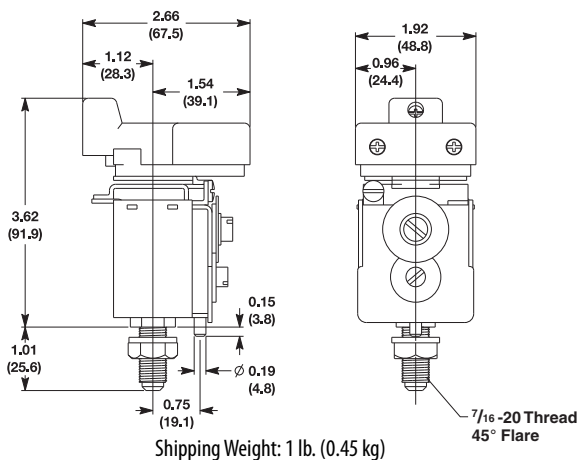
Figure 17 - Open Type
