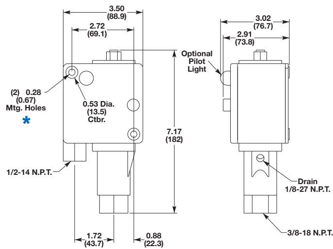
Figure 62 - Type 4 & 13 (Piston)
