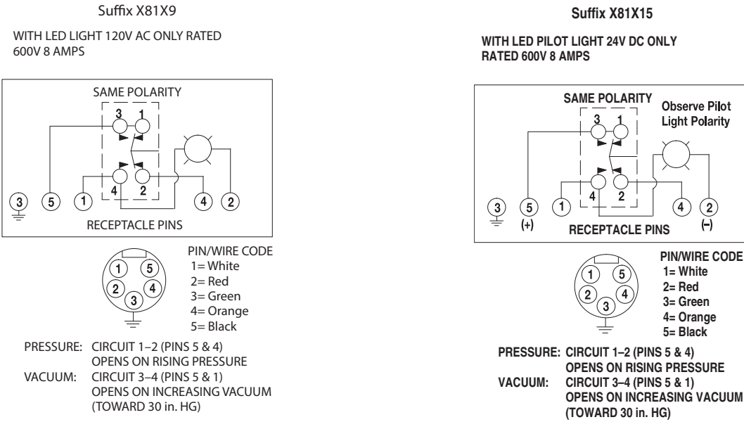
Figure 56 - With Pilot Light (2)
