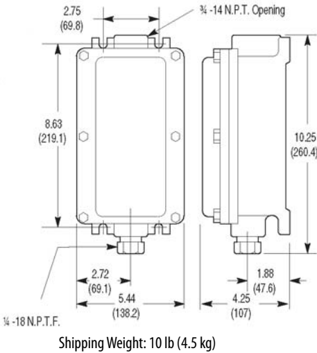
Figure 27 - Type 4X
