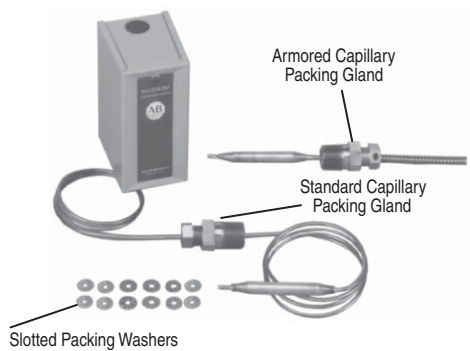
Figure 71 - Packing Glands
