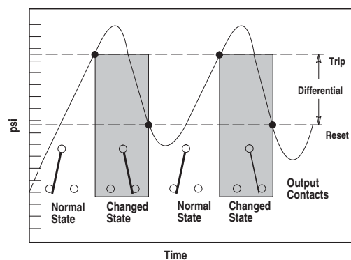
Figure 5 - Typical Monitoring Application
