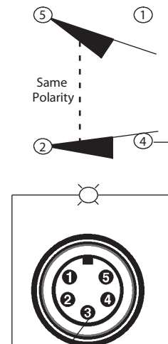
J9 Wiring Light Wired to N.C.
