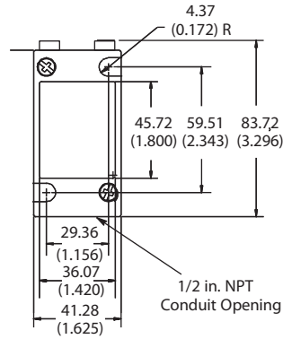
Switch Body
