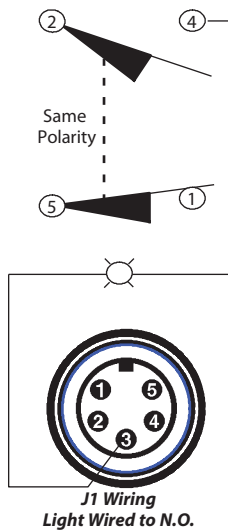
J1 Wiring Light Wired to N.O.
