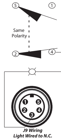
J9 Wiring Light Wired to N.C.
