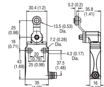
Lever Type
