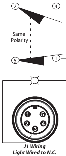
J1 Wiring Light Wired to N.C.
