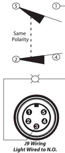
J9 Wiring Light Wired to N.O.
