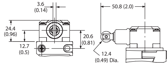
Plug-In Switch
