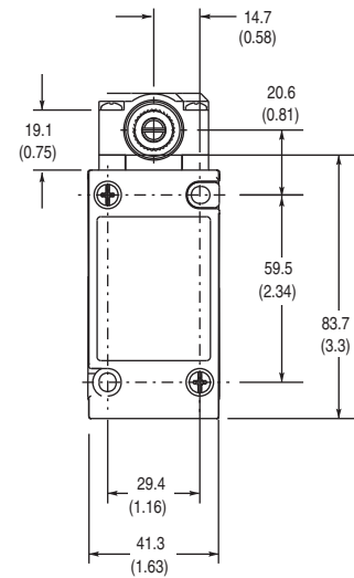
Plug-In Switch
