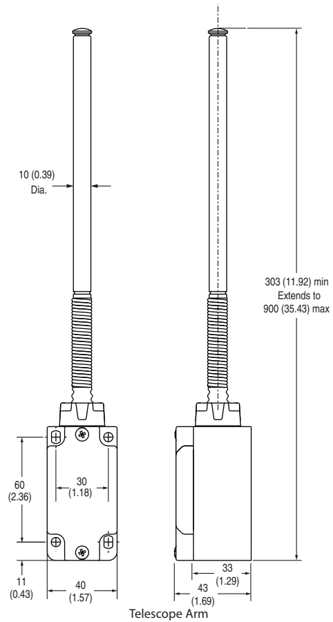
Telescope Arm
