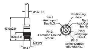
5-pin Micro Quick Disconnect
