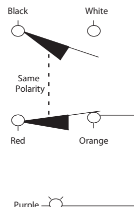
Light Wired to N.C. (Orange) Wire
