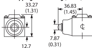
802T-C Side Push Rod Head Shipping Wt. 0.128 kg (4.5 oz)
