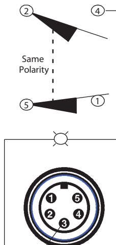
J1 Wiring Light Wired to N.O.
