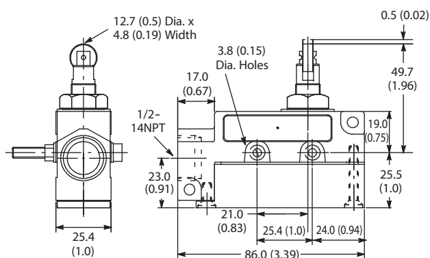
Cat. No. 802B-PSABXSX
