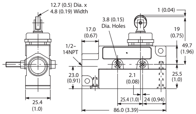
Cat. No. 802B-PSADBSX
