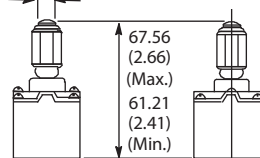
802T-BA Adjustable Top Push Rod Head Shipping Wt. 0.128 kg (4.5 oz)
