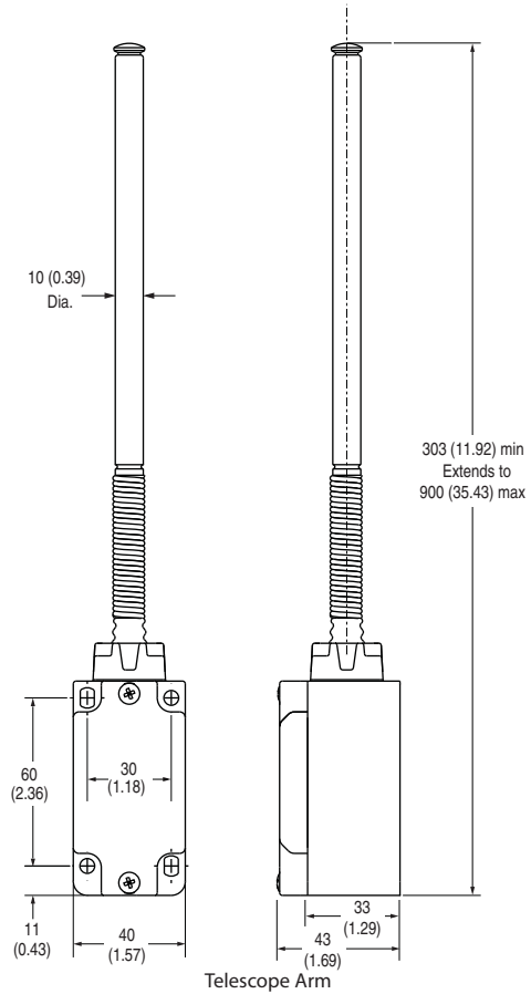
Telescope Arm
