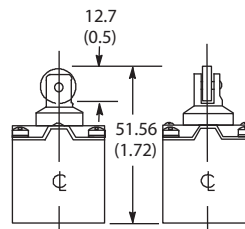
Z-36618 Top Push Roller Head Shipping Wt. 0.12 kg (4.25 oz)
