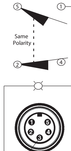
J9 Wiring Light Wired to N.O.
