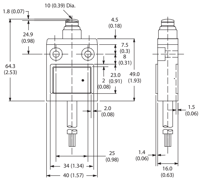
Top Push Booted Head
