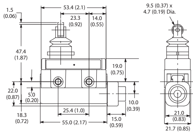
Cat. No. 802B-SSAD1BSX
