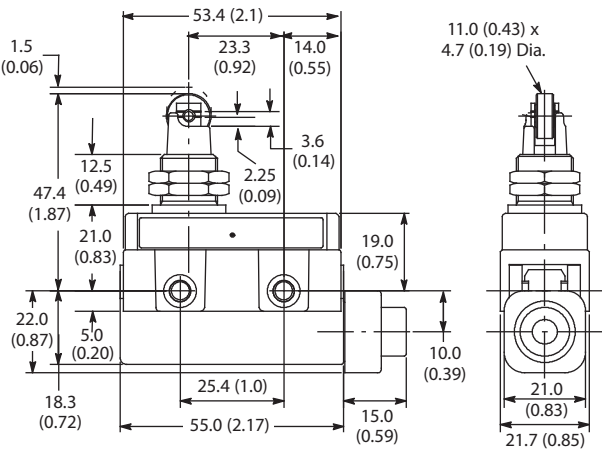
Cat. No. 802B-SPADX SX
