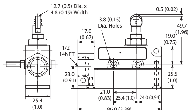
Cat. No. 802B-PSADXSX
