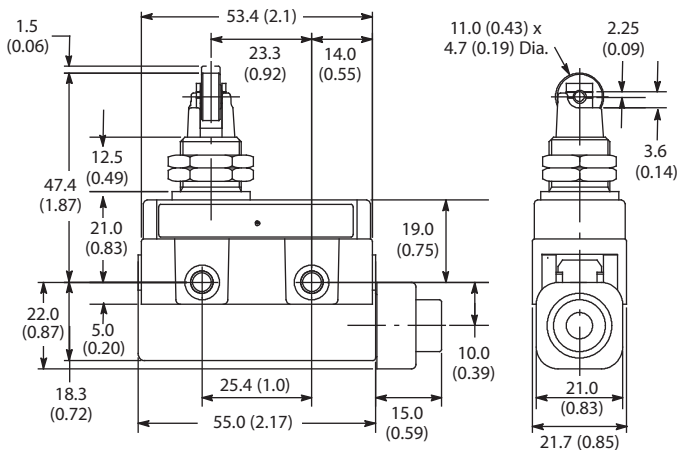
Cat. No. 802B-SPAD1XSX
