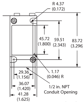
Switch Body
