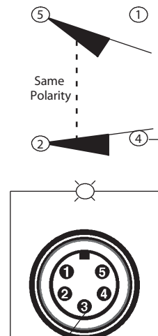
J9 Wiring Light Wired to N.C.
