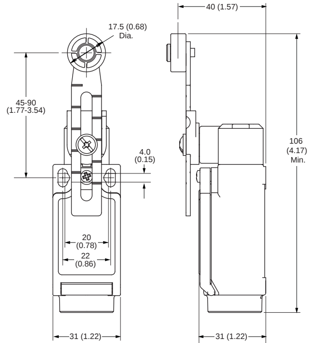
Adjustable Lever
