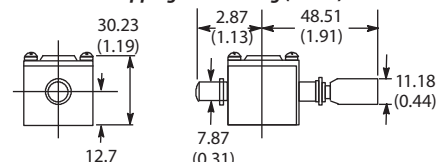
802T-CM Maintained Side Push Rod Head Shipping Wt. 4.5 oz (0.128 kg)
