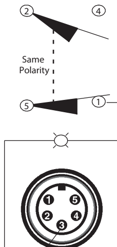
J1 Wiring Light Wired to N.C.
