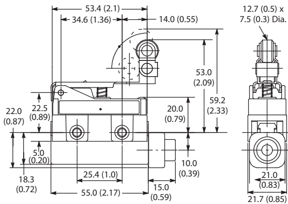
Cat. No. 802B-SSAR3XSX
