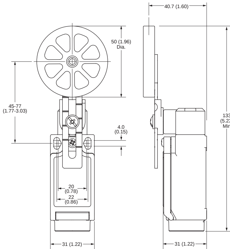
Rubber Roller
