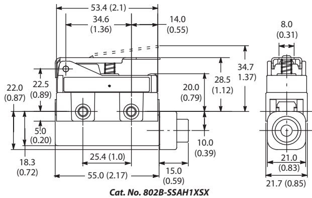
Cat. No. 802B-SSAH1XSX
