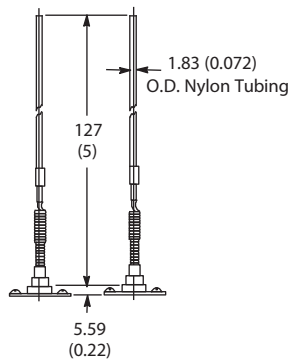
Z-35607 Cat Whisker Head Shipping Wt. 0.3 kg (1 oz)
