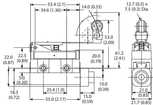
Cat. No. 802B-SSAR2XSX
