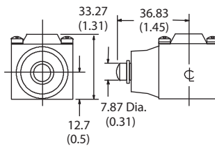
Z-36616 Side Push Rod Head Shipping Wt. 0.12 kg (4.25 oz)
