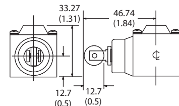
Z-36622 Side Push Vertical Roller Head Shipping Wt. 0.12 kg (4.25 oz)
