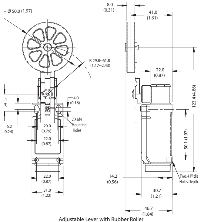
Adjustable Lever with Rubber Roller
