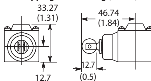
802T-K Side Push Roller Head Shipping Wt. 0.128 kg (4.5 oz)
