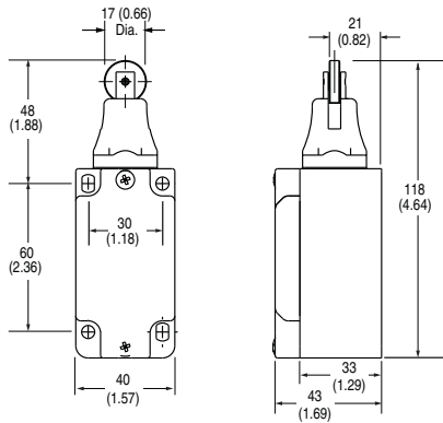
Roller Plunger
