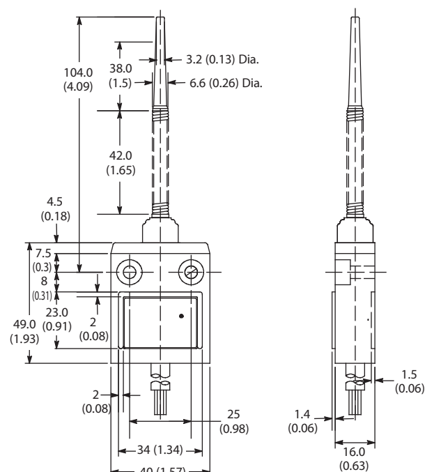
Wobble Stick
