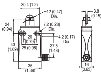
Roller Plunger
