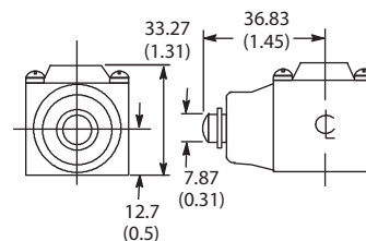
Cat. No. 802T-CT Side Push Rod Head
