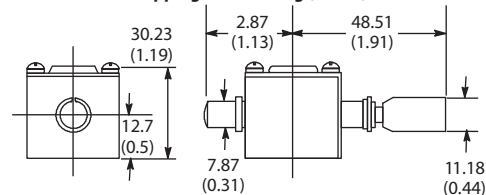
Cat. No. 802T-CMT Maintained Side Push Rod Head
