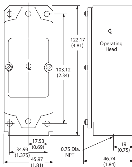
NonPlug-in Switch
