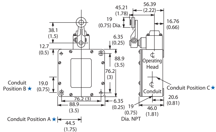
2-Pole Horizontal Switch with 802T-W1 Lever Shipping Wt. 0.91 kg (2 lb)
