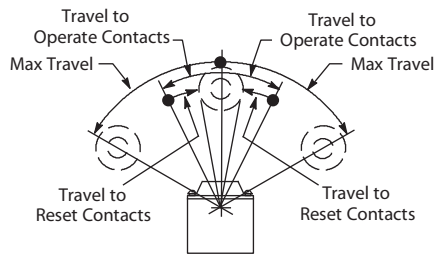
Lever Operation When Standard Levers Are Used
