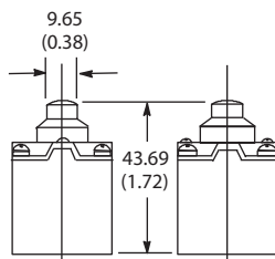
Cat. No. 802T-BT Top Push Rod Head
