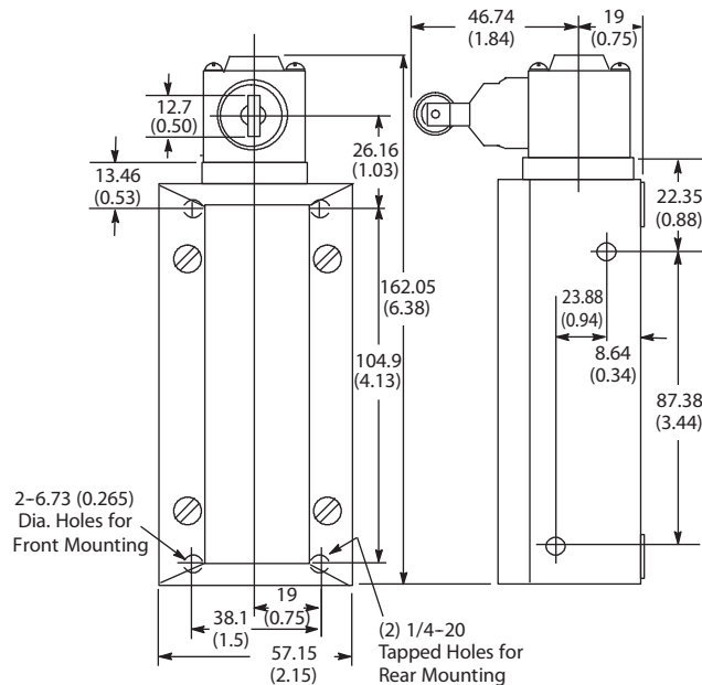
Bulletin 802XR Side Push Rod Type Approximate Shipping Wt. 0.9 kg (2 lb)
