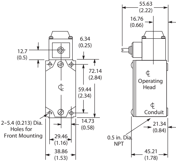
NonPlug-In Switch Shipping Wt. 0.45 kg (1 lb)
