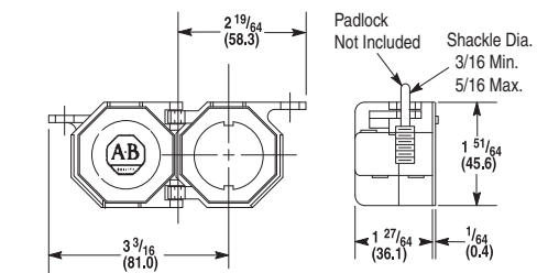
800H-N140 Locking Cover for 2-position Non-illuminated Maintained Twist or Pull Release and Standard Knob Selector Switch (1-5/8 (41.3) Mushroom Head only)
