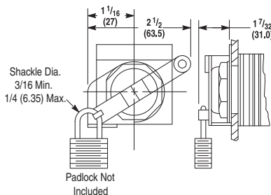
Locking Attachment for Extended, Non-illuminated Push Buttons
