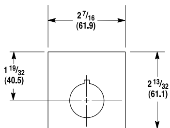
Type 4/4X Large Legend Plate (Automotive Industry Type)
