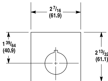
Large Size Push-pull/Twist Legend Plate Cat. No. 800T-X647 (1)
