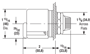
Push Button with Cylinder Lock Shipping Weight 12 oz (0.34 kg)
