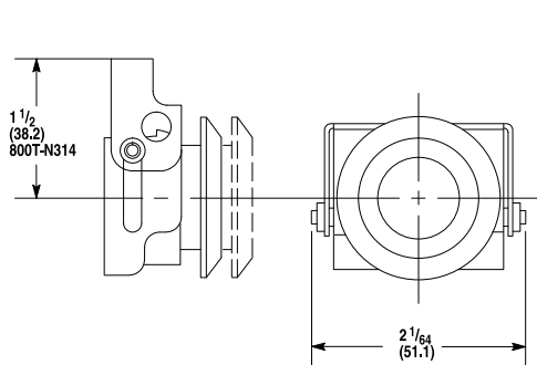
Push-pull/Twist Padlocking Attachment
