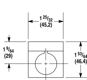
Standard Legend Plate
