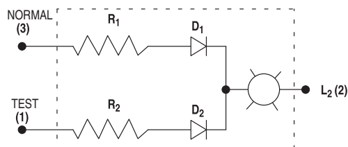
Dual-input Diode Pilot Light Device Schematic
