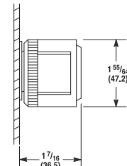
Protective Ring and Push-pull Illuminated or Non-illuminated Operators
