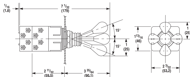
2-3-4 Way Switch Shipping Weight with Two Contact Blocks 6 oz (0.17 kg), with Four Contact Blocks 8-1/2 oz (0.24 kg)
