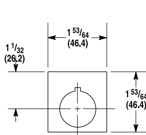
Type 4/4X Standard Legend Plate
