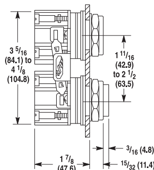
Mechanically Interlocked Maintained Contact Push Button Shipping Weight 1 lb (0.45 kg)
