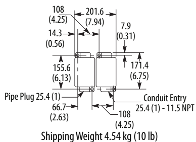
Control Station, 2-Gang (up to four devices)
