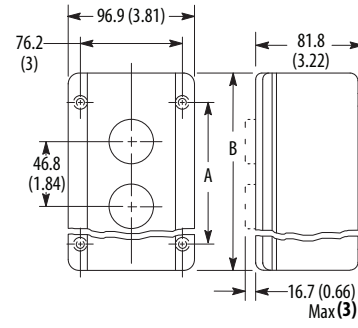
Type 4/13 Cast Aluminum Enclosure Watertight/Oiltight
