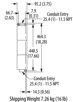
Control Station, 4-Gang (up to eight devices)
