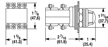
Cluster Pilot Light Shipping Weight 12 oz (0.34 kg)
