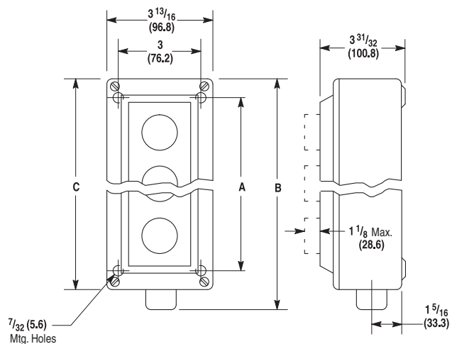
Type 4/4X/13 Rosite Glass Polyester Watertight, Oiltight, Corrosion-resistant Enclosure
