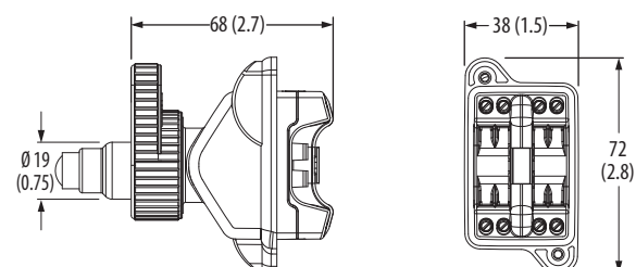
Screw Termination (-Ex models only)
