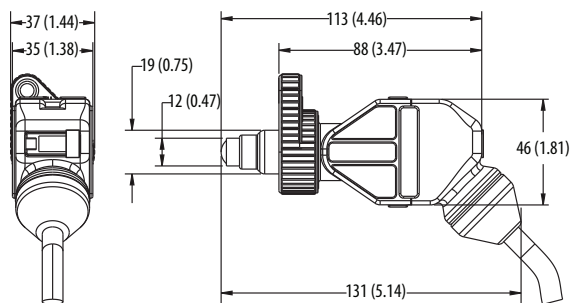
Cable Termination (c-UL-us models only)
