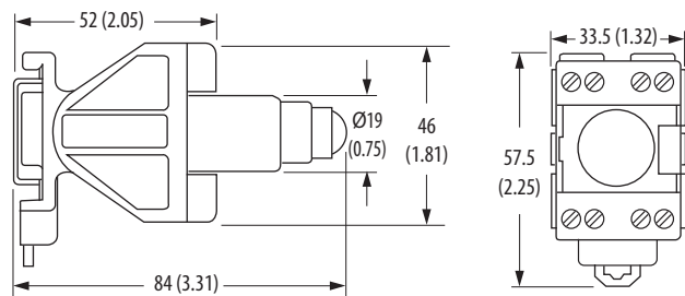
Base Mount
