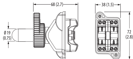
Screw Termination (-Ex models only)
