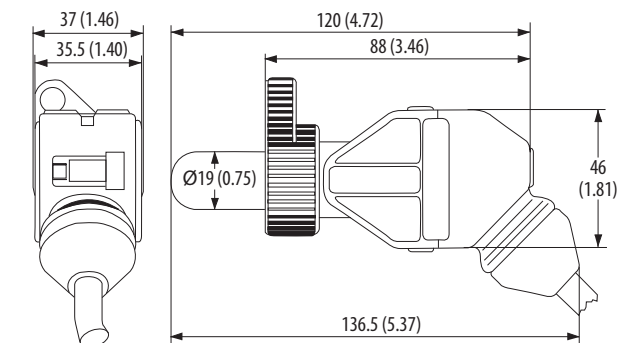
Cable Termination (c-UL-us models only)
