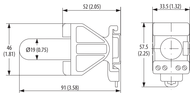
Base Mount
