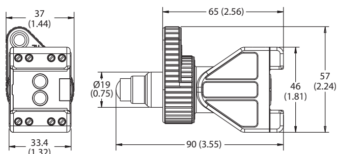
Latch Mount (c-UL-us models only)
