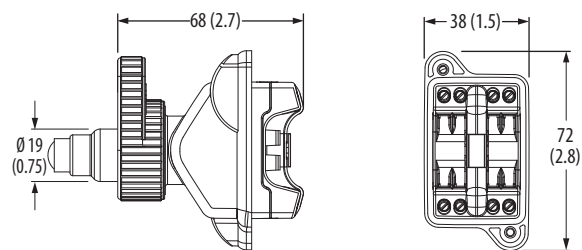
Screw Termination (-Ex models only)
