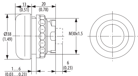
Push Buttons
