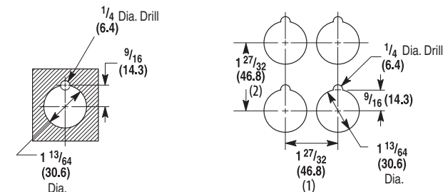
Figure 2 - Minimum Distance Between Centerlines
