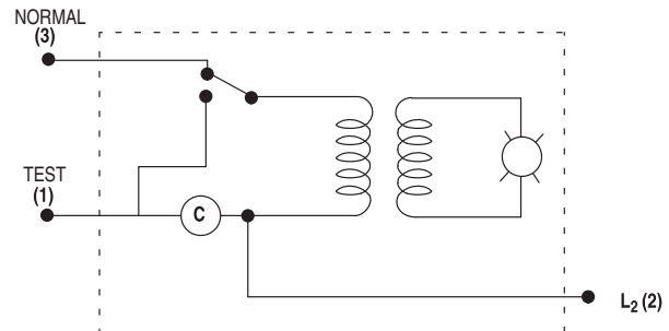
Dual-input Pilot Light Transformer Type Device Schematic
