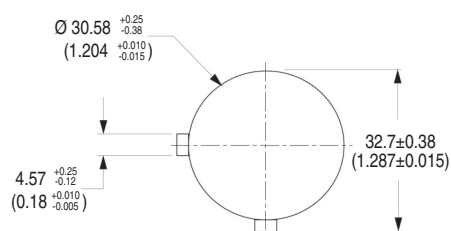
30.5 mm Push Button Hole
