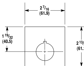
Type 4/4X Large Legend Plate (Automotive Industry Type)
