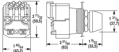
Dual-input Transformer Type Pilot Light
