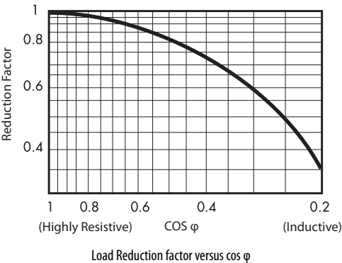
Load Reduction factor versus cos φ
