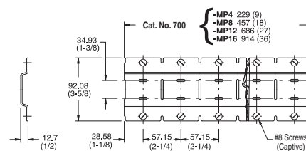
Relay Rail
