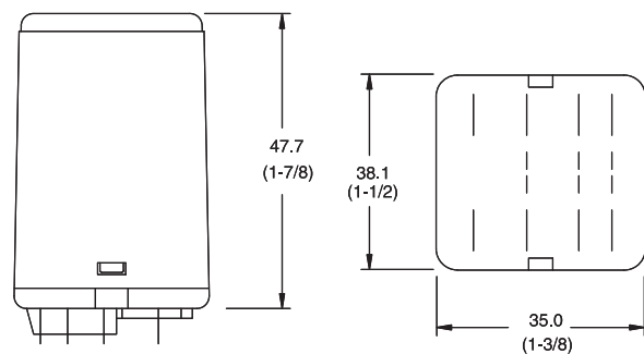
700-HJ Relay
