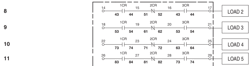
(5) Output Circuit (3 Relays, 17 Terminal Blocks)
