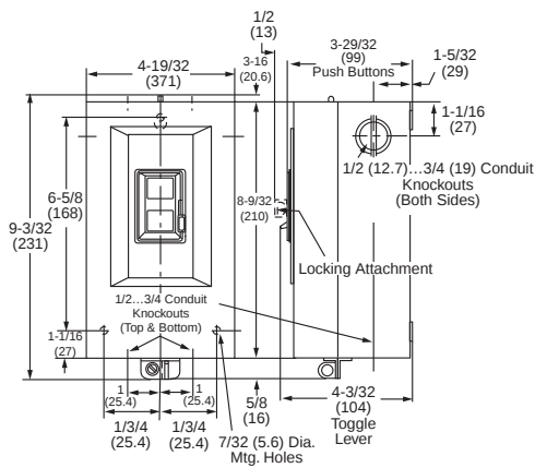
Surface Mounting
