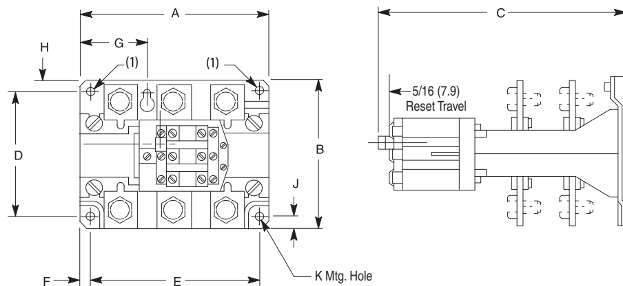
Figure 2 - Open Type without Enclosure for Bulletin 592 Current Transformer Type — Eutectic Alloy, Manual Reset
