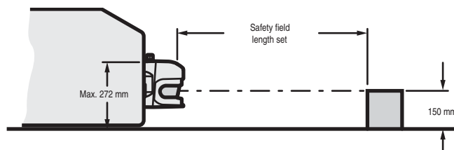
Figure 35: Mounting height
