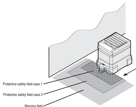
Figure 11: Field switching
