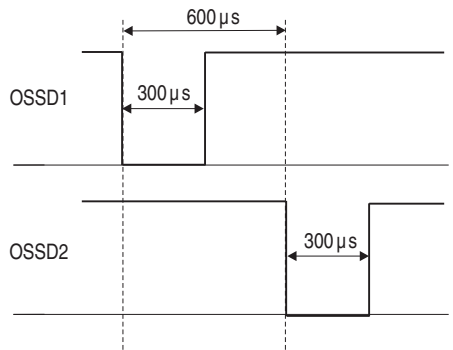
Figure 67: Voltage Test
