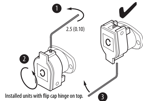
Figure 2 - Assembly
