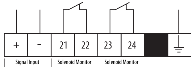
Figure 4 - Signal Input
