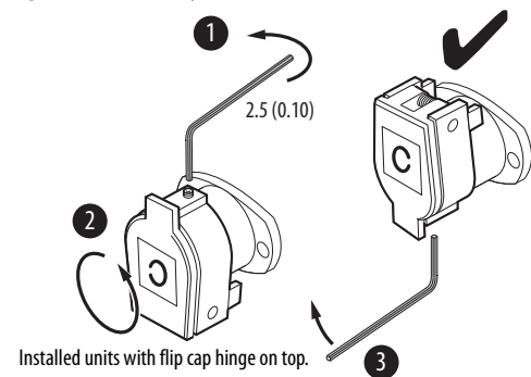
Figure 2 - Assembly
