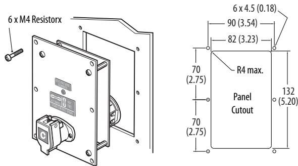
Figure 2 - Assembly
