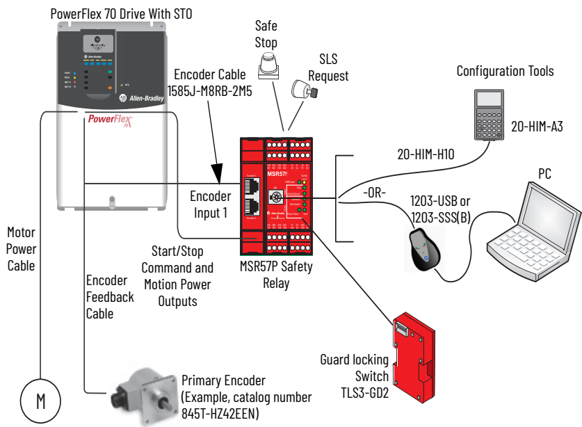
Figure 5 - System Layout
