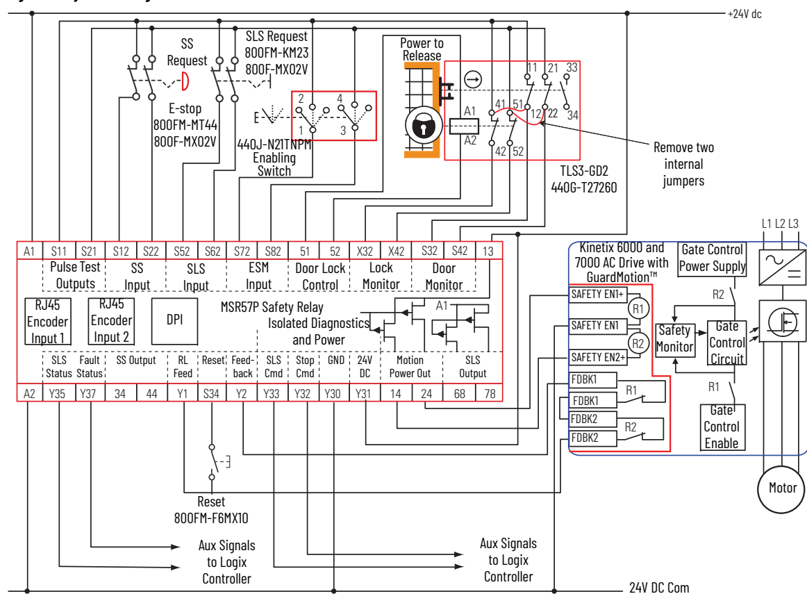
Figure 9 - System Wiring
