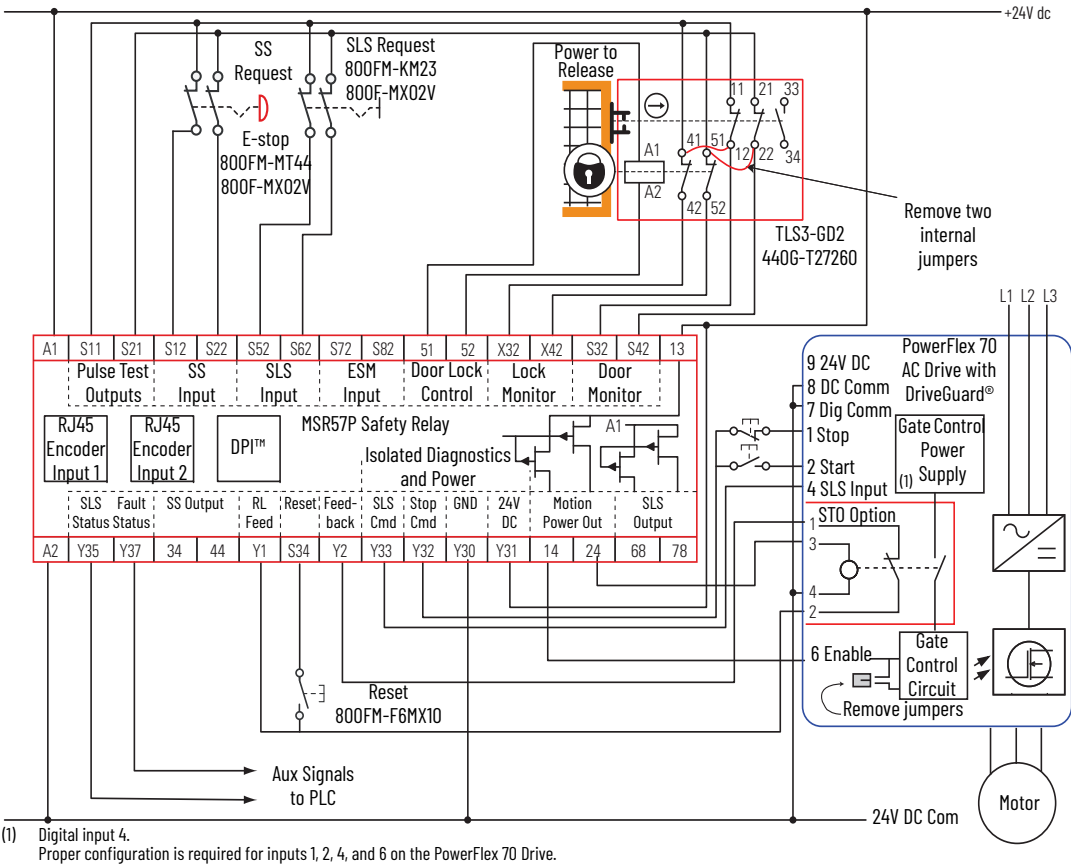
Figure 6 - System Wiring
