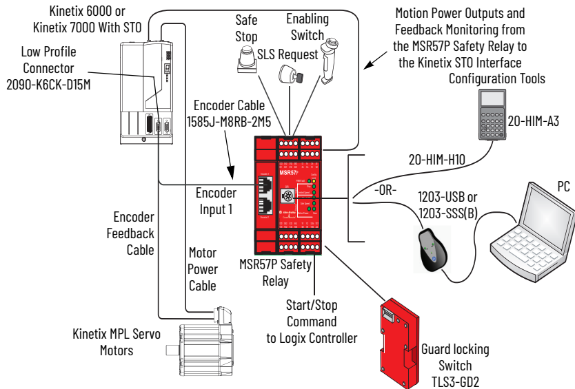
Figure 8 - System Layout
