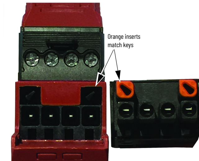
Figure 92 - Orange Keyway
