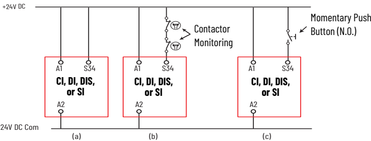
Figure 22 - Automatic/Manual Reset Connections
