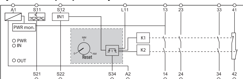
Figure 37 - CI Safety Relay Circuit Diagram
