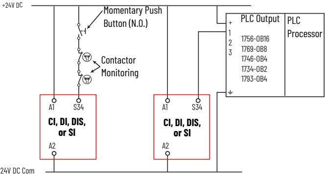
Figure 24 - Monitored Reset Connections
