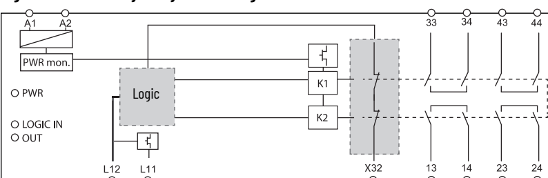
Figure 40 - EM Safety Relay Circuit Diagram
