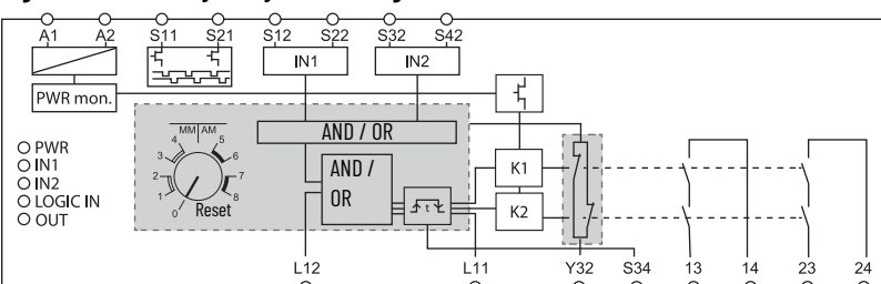
Figure 38 - DI Safety Relay Circuit Diagram
