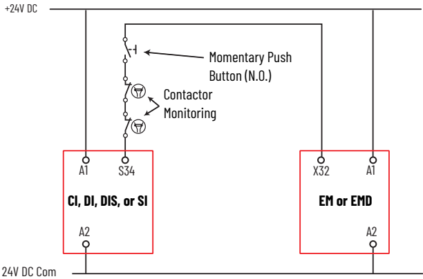
Figure 25 - Monitor Expansion Relay
