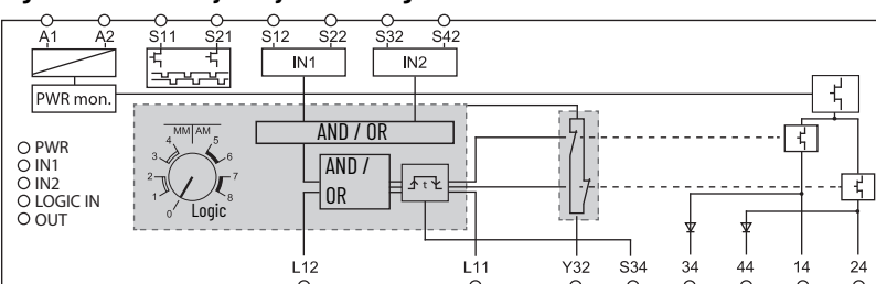
Figure 39 - DIS Safety Relay Circuit Diagram
