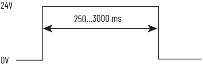
Figure 23 - Monitored Reset Signal Duration
