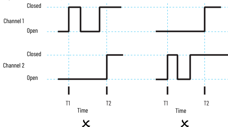
Figure 71 - Multiple Cycles on One Channel Are Not Allowed
