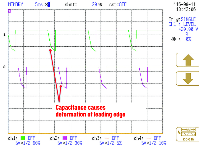
Figure 68 - Capacitive Effect on Pulse Tests
