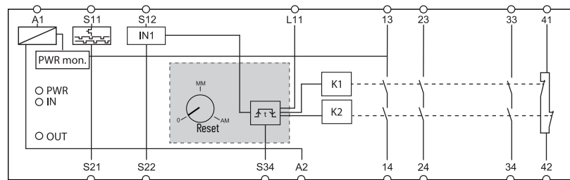
Figure 37 - CI Safety Relay Circuit Diagram
