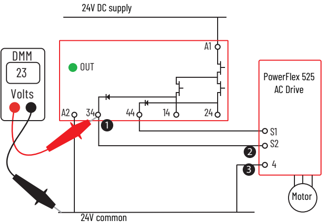
Figure 82 - Typical Connections to PowerFlex Drive
