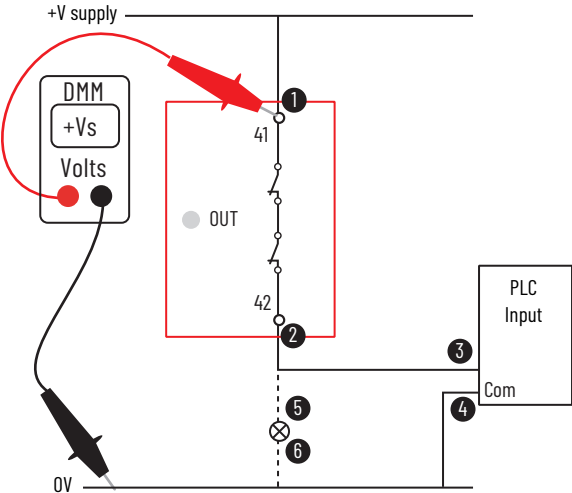
Figure 86 - Measure Voltage Aux Output Terminals
