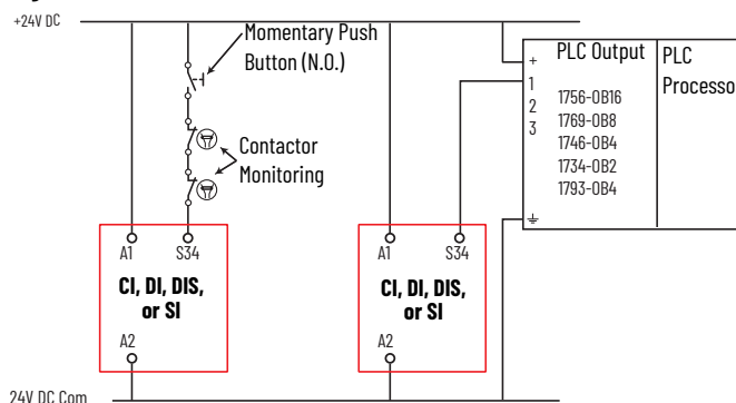
Figure 24 - Monitored Reset Connections
