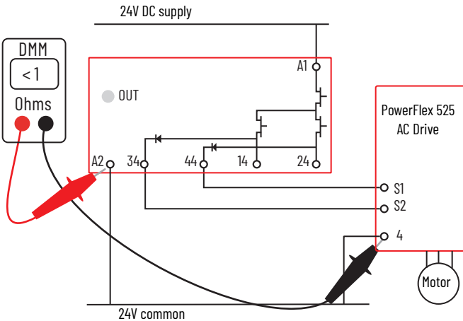
Figure 83 - Continuity Test of the Voltage Supply Common Connection
