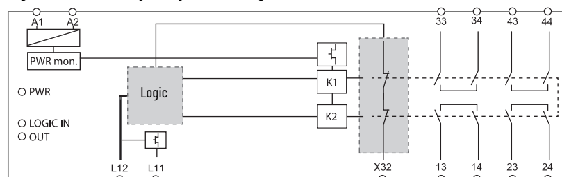
Figure 40 - EM Safety Relay Circuit Diagram
