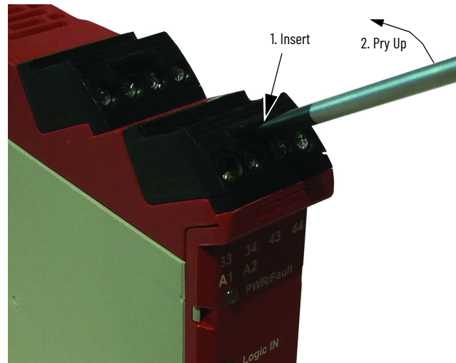
Figure 91 - Terminal Block Removal
