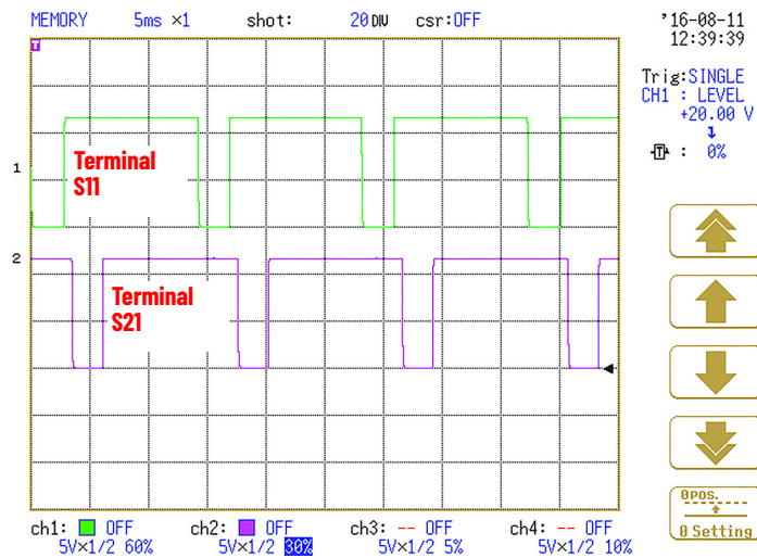
Figure 66 - CI Safety Relay Pulse Test Waveforms
