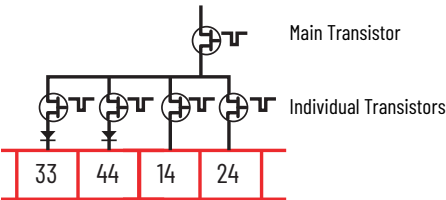
Figure 31 - Output Transistor Arrangement
