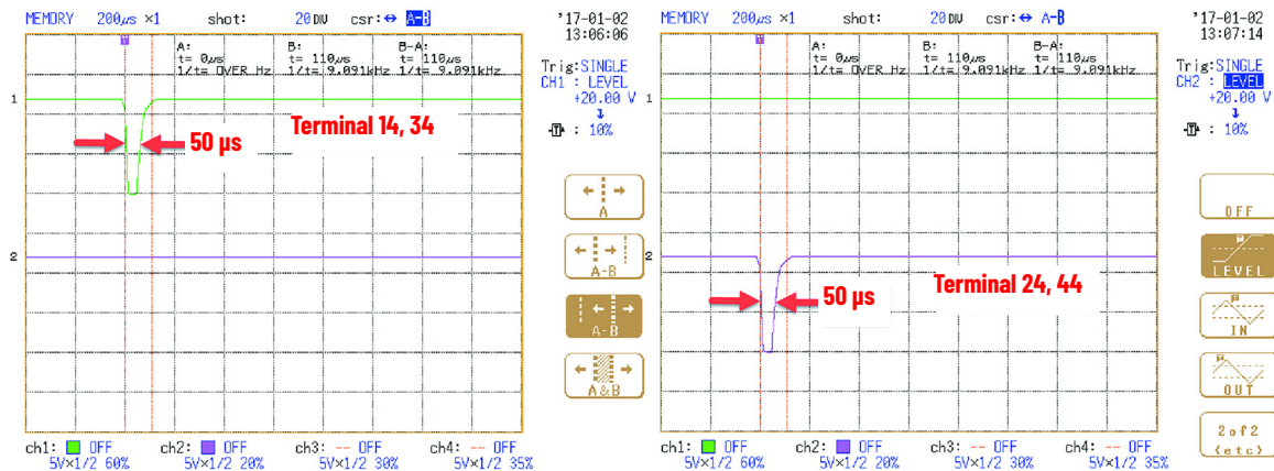
Figure 85 - OSSD Channel Transistor Test Pulse
