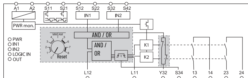
Figure 38 - DI Safety Relay Circuit Diagram
