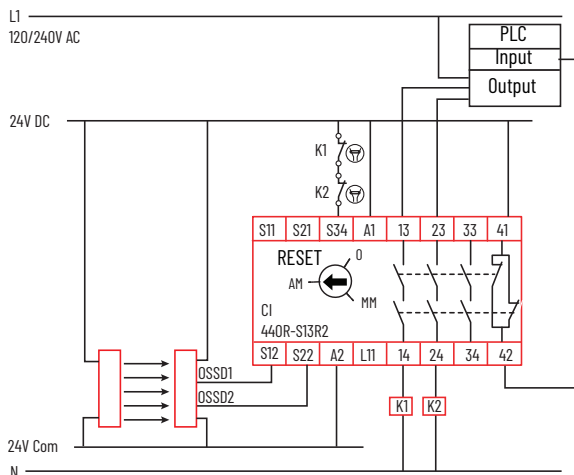
Figure 44 - With Device Using OSSD Outputs, Automatic Reset, AC Load Voltage
