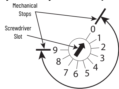
Figure 26 - Configuration Switch Adjustment
