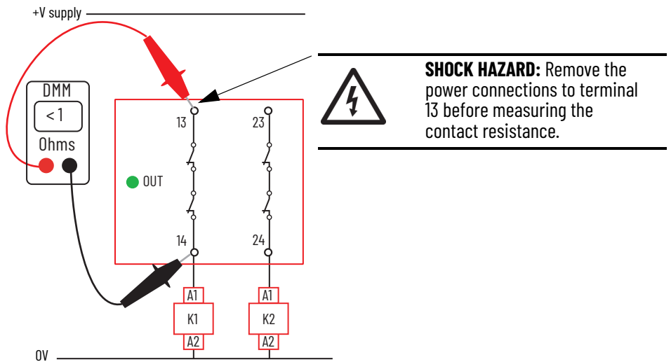
Figure 80 - Measure the Contact Resistance
