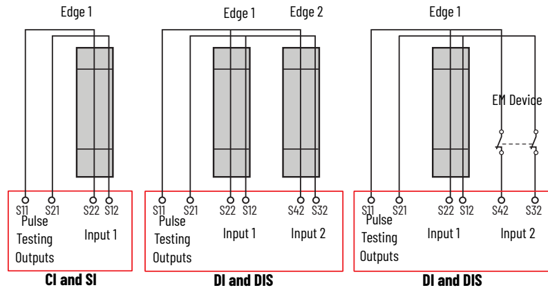
Figure 15 - Example Connections to Safety Edges
