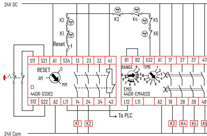
Figure 50 - EMD Safety Relay - Off Delay
