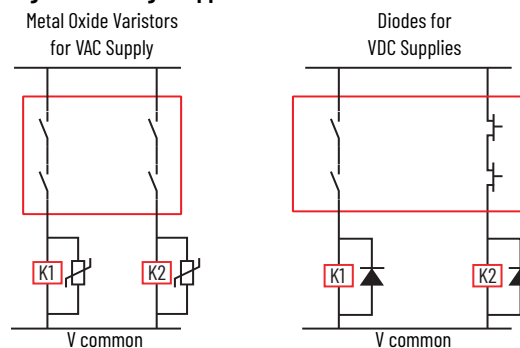
Figure 18 - Surge Suppressors
