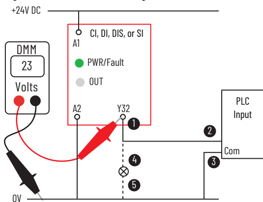
Figure 88 - Measure Y32 Voltage
