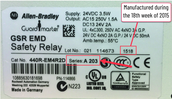
Figure 93 - Product Label - Series and Revision Identification
