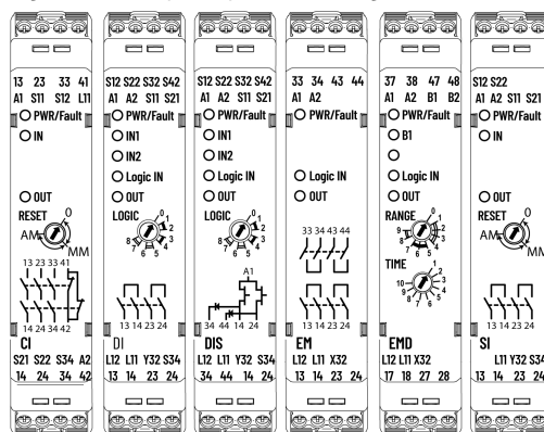
Figure 6 - Safety Relay Face Markings
