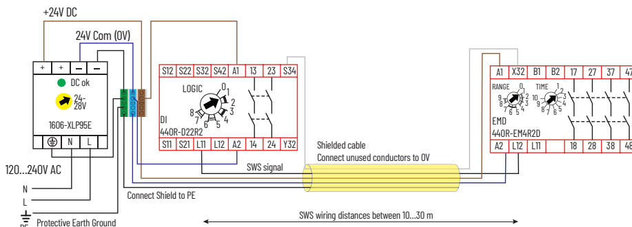
Figure 74 - SWS with Shielded Cable
