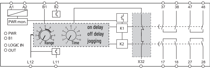
Figure 41 - EMD Safety Relay Circuit Diagram
