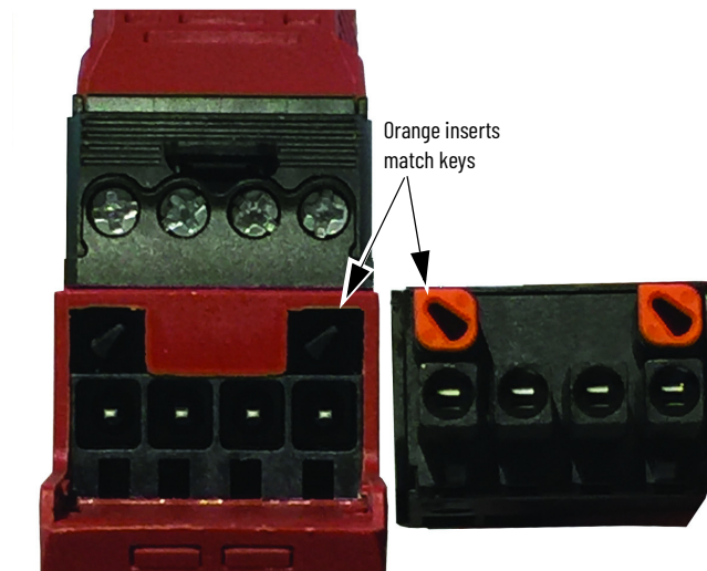
Figure 92 - Orange Keyway
