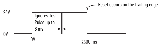
Figure 78 - Reset Input Ignores Test Pulses Up to 6 ms
