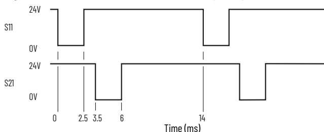
Figure 29 - Pulse Test Sequence for CI Safety Relay
