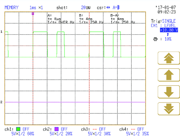
Figure 90 - The B1-B2 Waveform When the EMD Safety Relay Output is On
