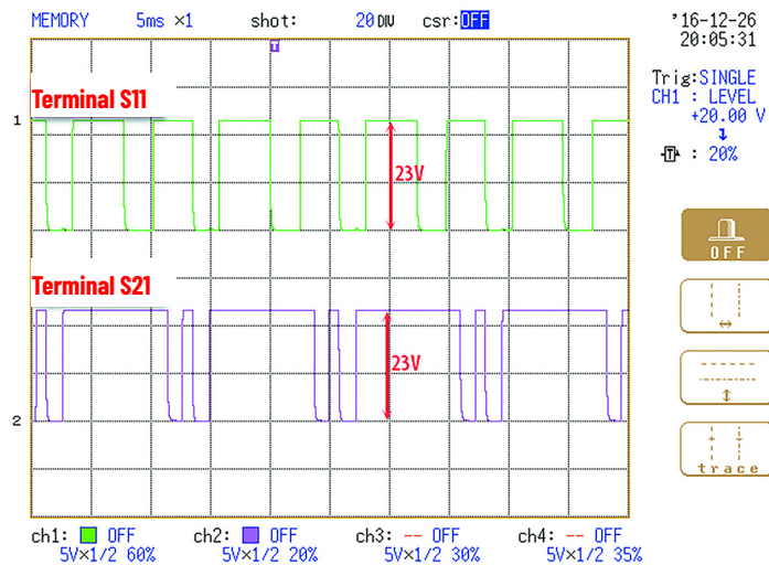
Figure 67 – DI, DIS, and SI Safety Relay Pulse Test Waveforms
