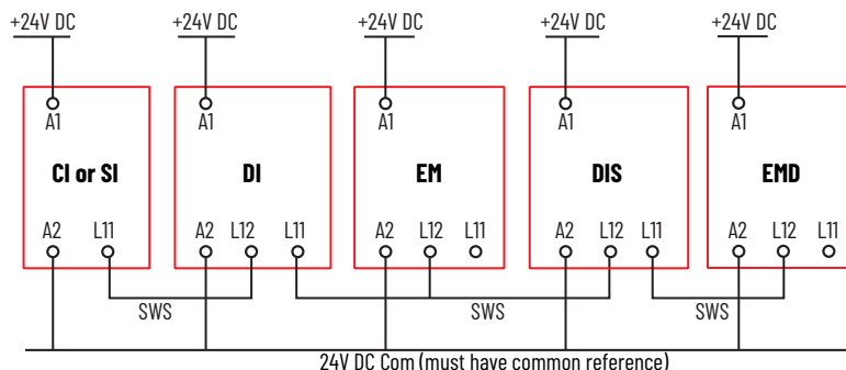
Figure 73 - Example SWS Connections
