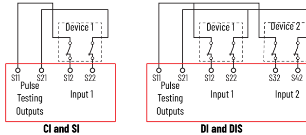
Figure 8 - Example Connections to 2 N.C. Mechanical Contacts
