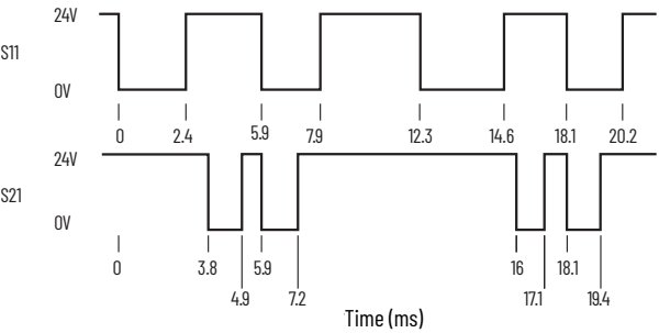
Figure 30 - Pulse Test Sequence for DI, DIS, and SI Safety Relays
