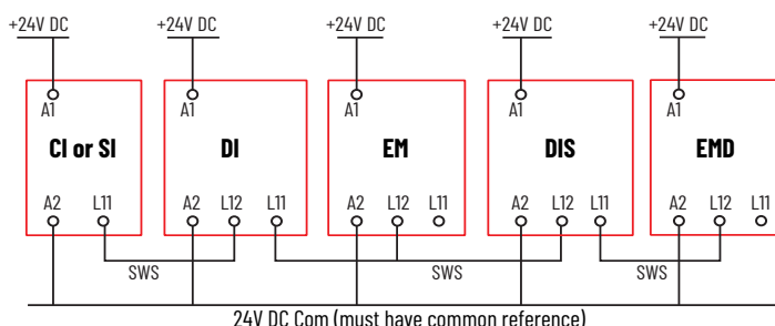
Figure 19 - Example SWS Connections
