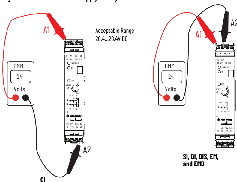
Figure 60 - Measure Power Supply Voltage
