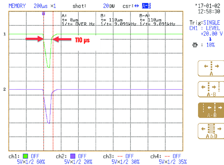
Figure 85 - OSSD Channel Transistor Test Pulse
