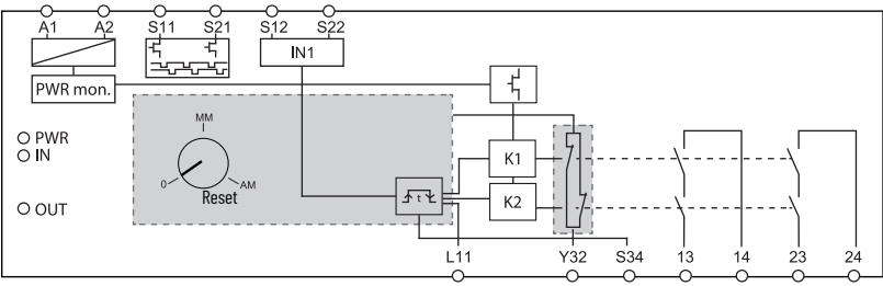
Figure 42 - SI Safety Relay Circuit Diagram
