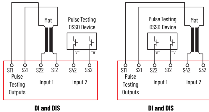
Figure 13 - Example Combining Safety Mats with Devices with OSSD Outputs
