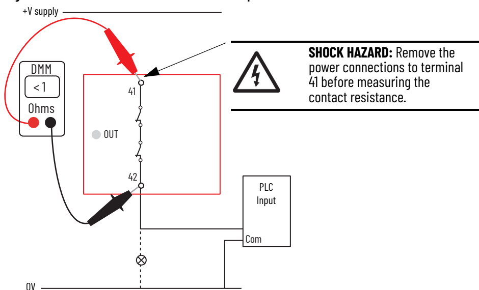
Figure 87 - Measure Contact Resistance of Aux Output Terminals
