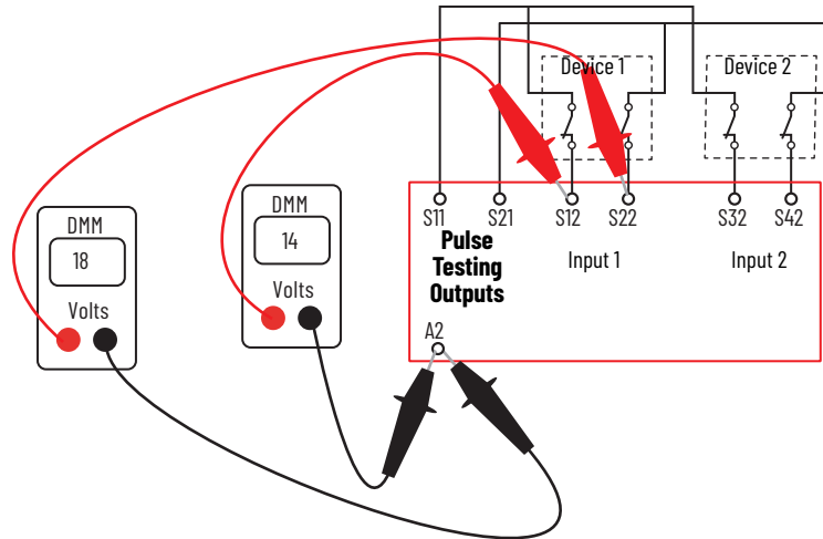
Figure 65 - Typical Voltage Measurements of the DI, DIS, and SI Safety Relays with Contacts Closed
