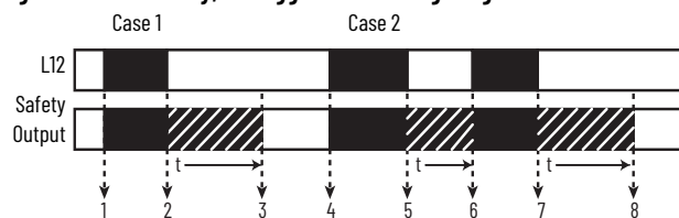
Figure 34 - Off-delay, Retriggerable Timing Diagram
