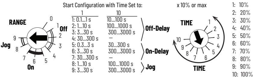
Figure 27 - EMD Safety Relay Range and Time
