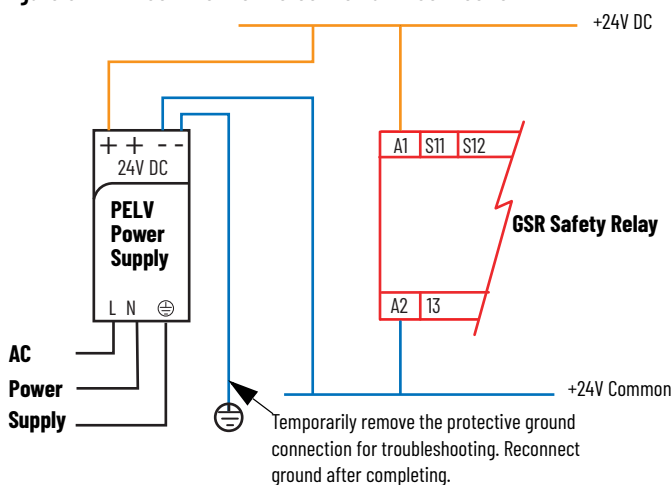
Figure 61 - 24V Common to Protective Earth Connection
