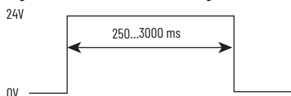
Figure 23 - Monitored Reset Signal Duration
