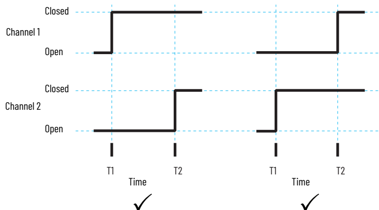
Figure 70 - GSR Safety Relays Have Infinite Simultaneity (Discrepancy)
