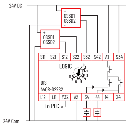
Figure 48 - High Capacitive Load
