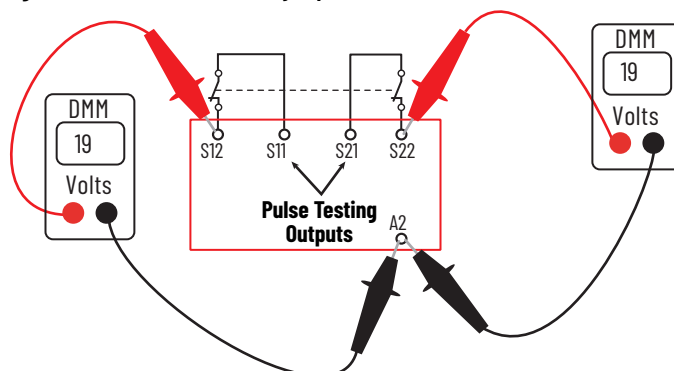
Figure 63 - Check the CI Safety Inputs with the Device Contacts Closed
