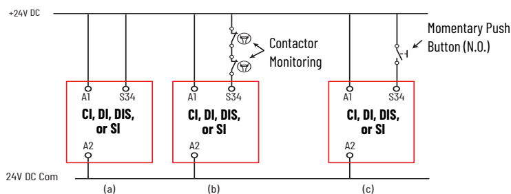
Figure 22 - Automatic/Manual Reset Connections
