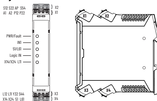
Figure 5 - Terminal Identification
