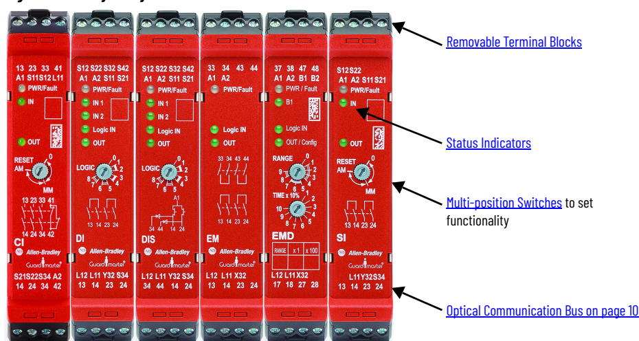
Figure 1 - Safety Relays
