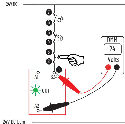
Figure 77 - Measure Reset/Monitoring Circuit Voltage
