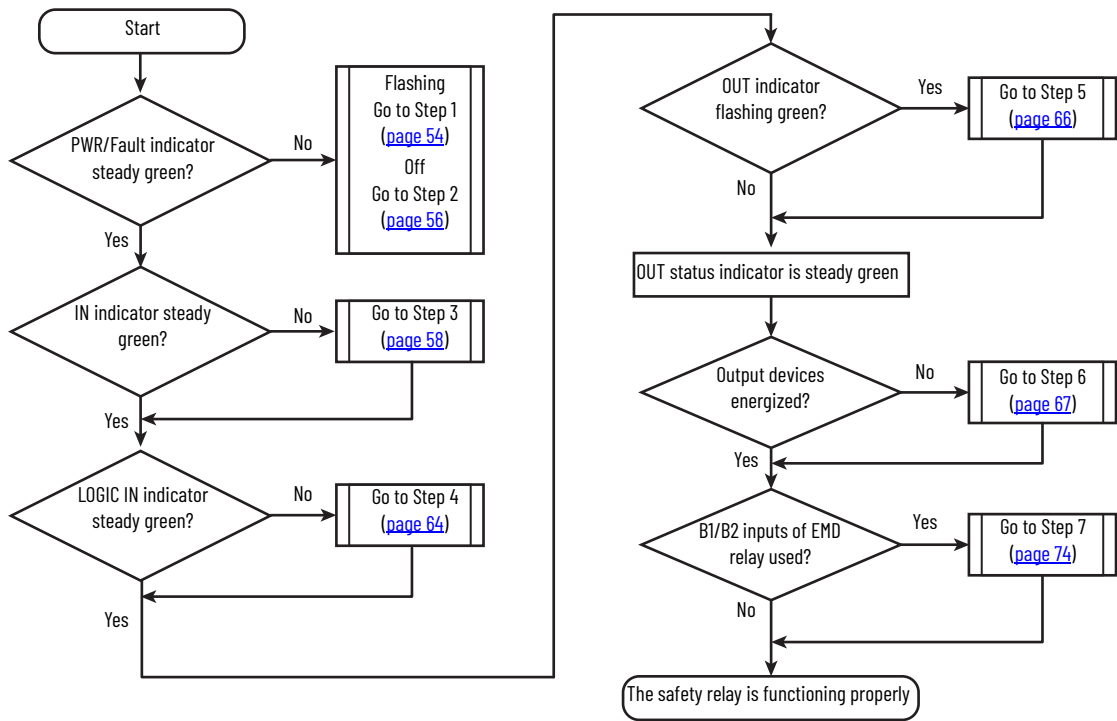
Figure 58 – Troubleshooting Flowchart
