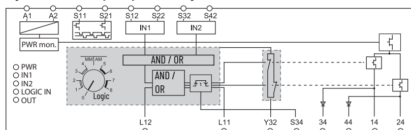
Figure 39 - DIS Safety Relay Circuit Diagram
