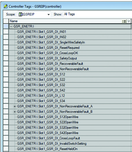
Figure 56 - AOP for the DI Safety Relay
