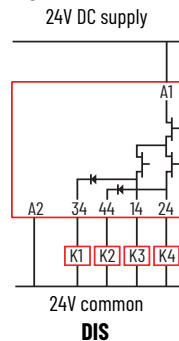
Figure 17 - OSSD Output Connections
