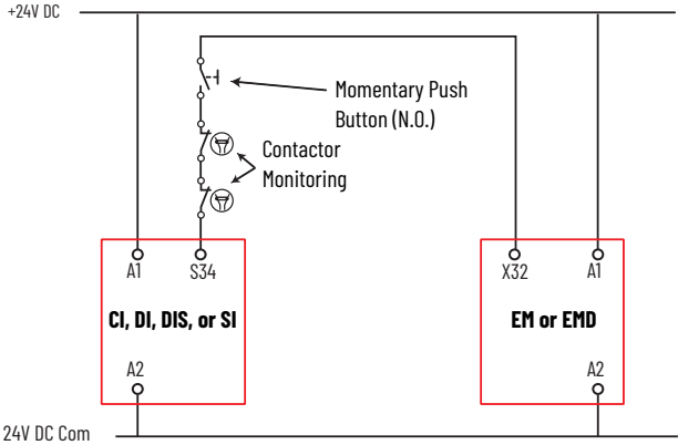
Figure 25 - Monitor Expansion Relay
