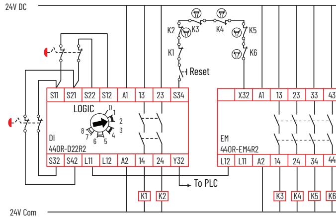
Figure 49 - Expansion of Immediate Safety Outputs
