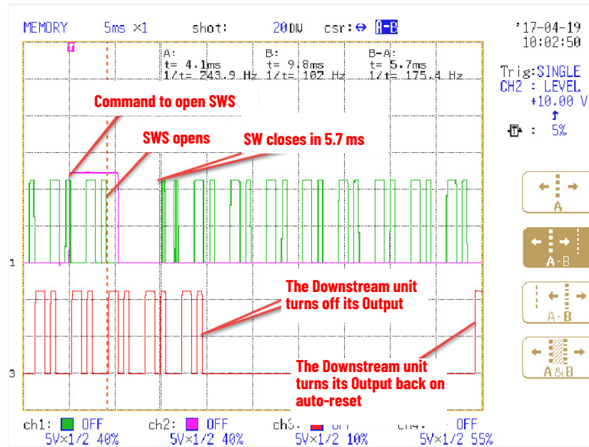
Figure 76 - Momentary Interruption of SWS Input
