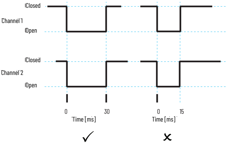
Figure 72 - Recovery Time
