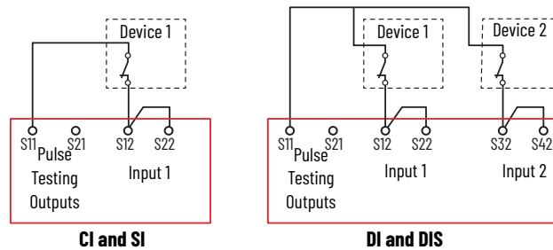
Figure 9 - Example Connections to 1 N.C. Mechanical Contact
