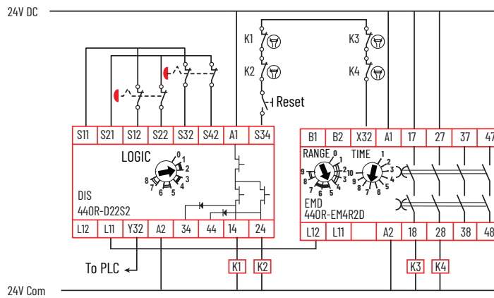
Figure 51 - EMD Safety Relay - On Delay
