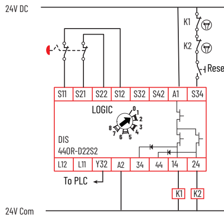
Figure 47 - Single Input, Monitored Reset
