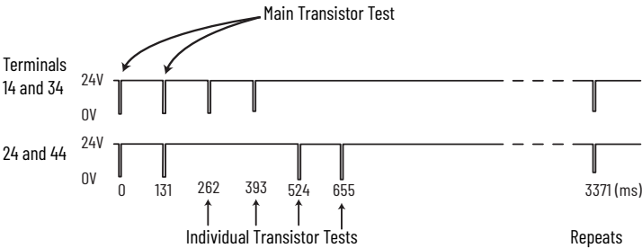
Figure 32 - OSSD Output Test Pulses on DIS Safety Relay
