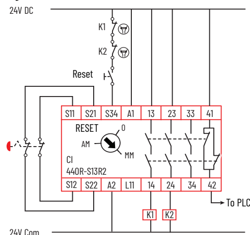
Figure 43 - Mechanical Contacts with Monitored Manual Reset
