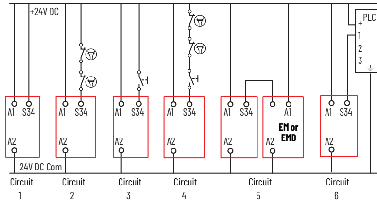
Figure 21 - Typical Reset/Monitoring Circuits
