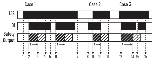
Figure 36 - Jog Timing Diagram
