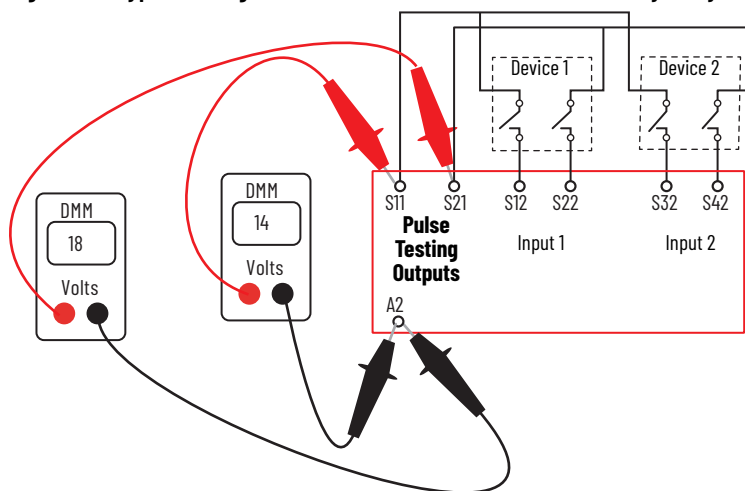
Figure 64 - Typical Voltage Measurements of the DI, DIS, and SI Safety Relays with Contacts Open
