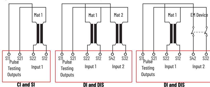
Figure 12 - Example One Connection to Safety Mats
