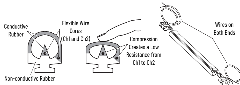
Figure 14 - Safedge Operating Principle
