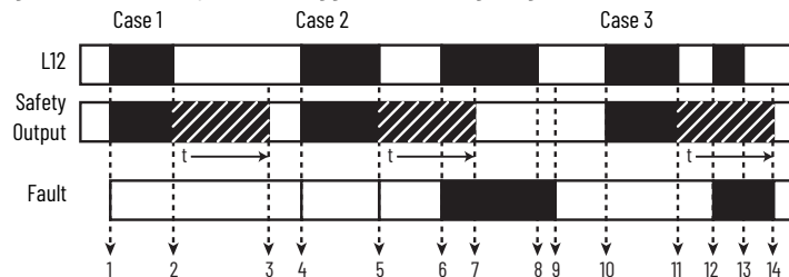
Figure 33 - Off-delay, Non-retriggerable Timing Diagram
