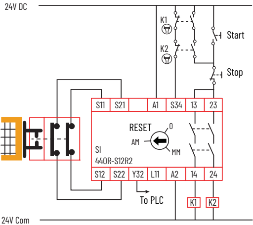
Figure 53 – SI Safety Relay Example
