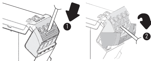
Figure 4 - Removable Terminals
