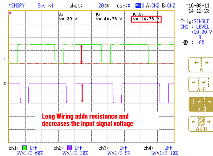
Figure 69 - Resistance Effect on Input Signal
