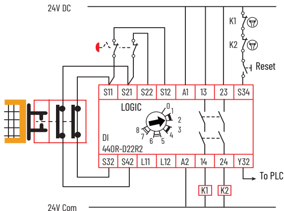
Figure 45 - With Two Devices with Mechanical Contacts and Monitored Manual Reset
