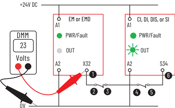
Figure 89 - Measure X32 Voltage
