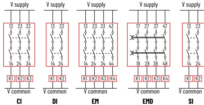
Figure 16 - Electromechanical Output Connections
