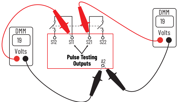
Figure 62 - Typical Voltage Measurements of the CI Safety Relay
