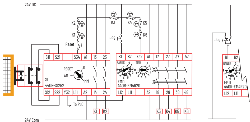
Figure 52 - EMD Safety Relay - Jog
