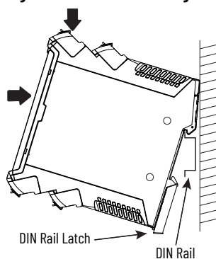
Figure 3 - DIN Rail Mounting
