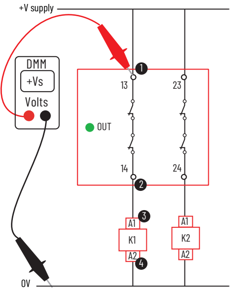
Figure 79 - Measure the Terminal Voltage
