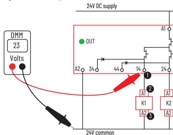
Figure 81 - OSSD Output Connections
