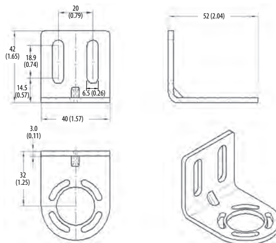
Figure 9: Mounting brackets
