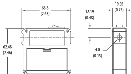
Laser Alignment Tool (LAT)—440L-ALAT
