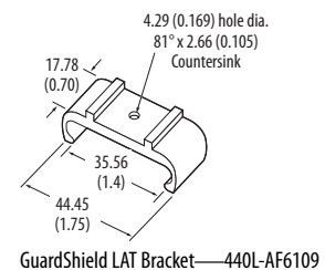
GuardShield LAT Bracket—440L-AF6109
