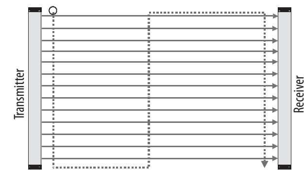
Figure 4: Proper testing of protective field using test rod
