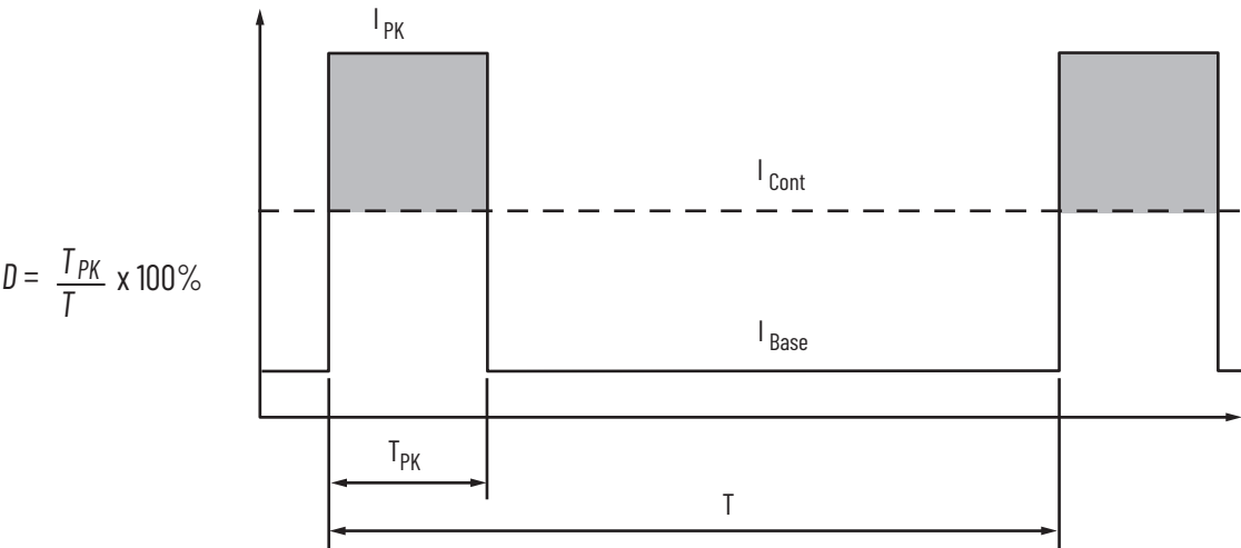
Load Duty-cycle Profile Example
