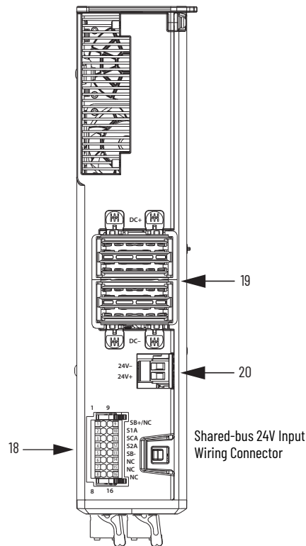
Dual Axis Inverter, Top View (Z198-D006-ERS4 module is shown)
