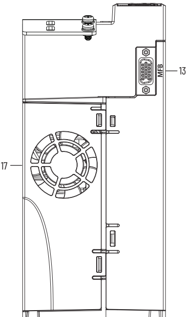
Kinetix 5100 Drive, Bottom View (2198-E1020-ERS drive is shown)
