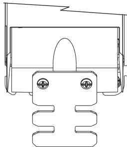
Frame 3 clamping plate for large diameter cables.
