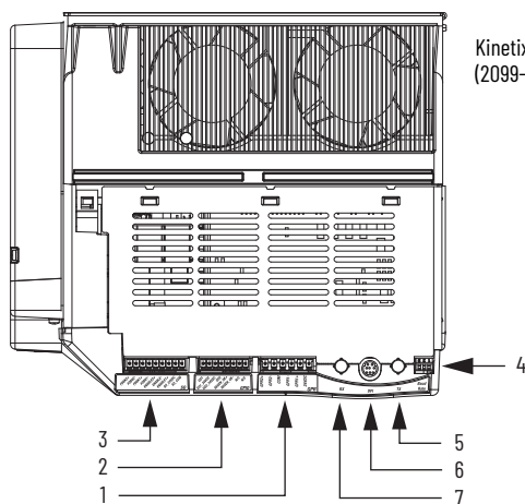
Kinetix 7000 Drive Module (2099-BM07-S front view is shown)
