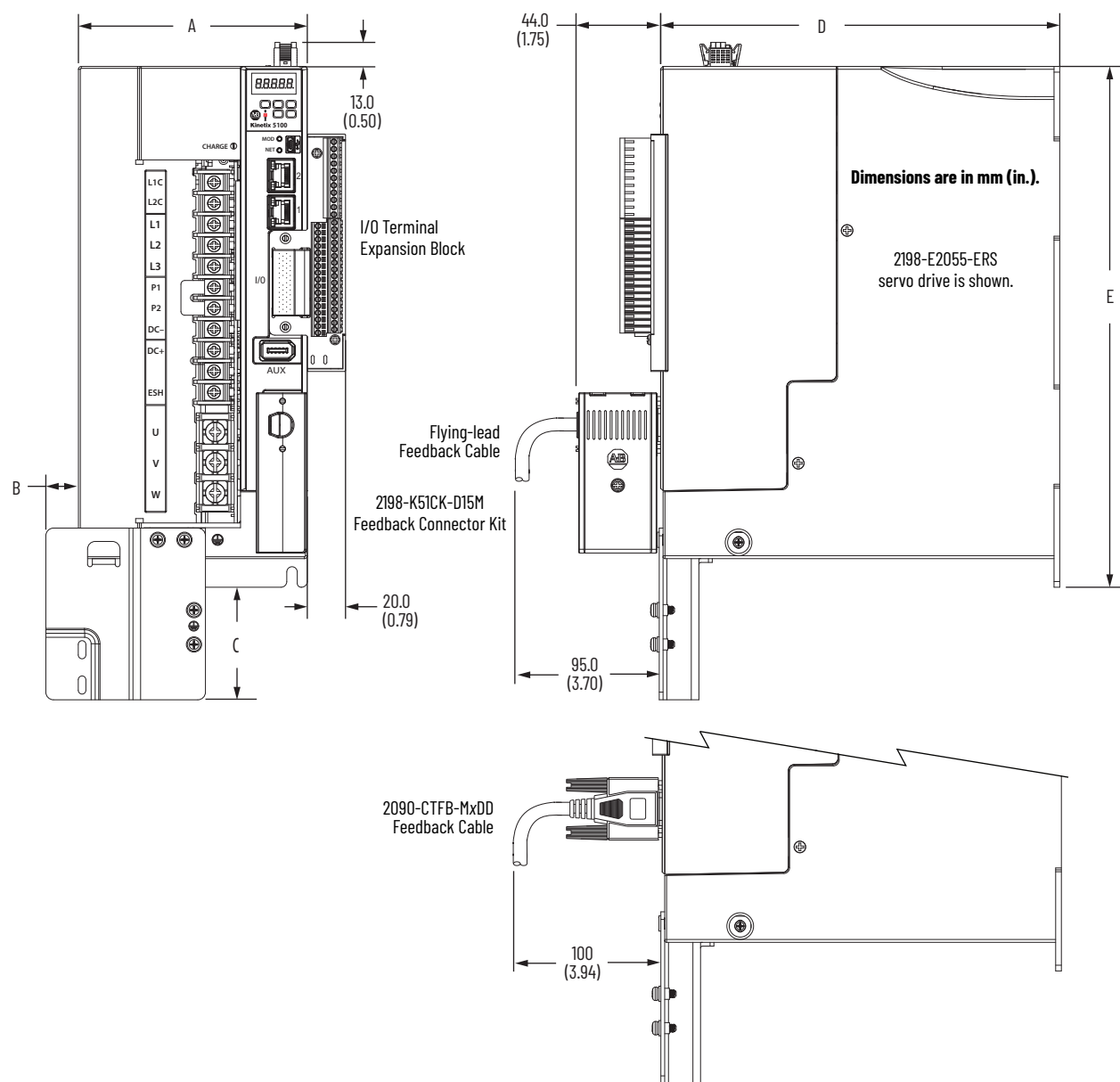
Kinetix 5100 Drive Dimensions
