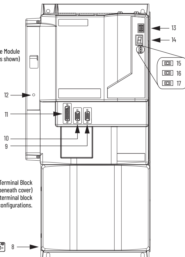
Kinetix 7000 Drive Module (2099-BM07-S top view is shown)
