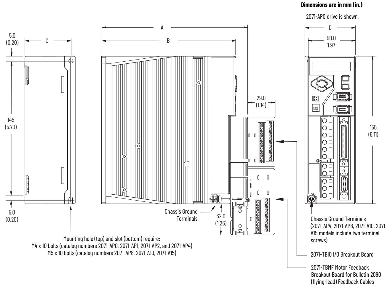
Kinetix 3 Drive Dimensions
