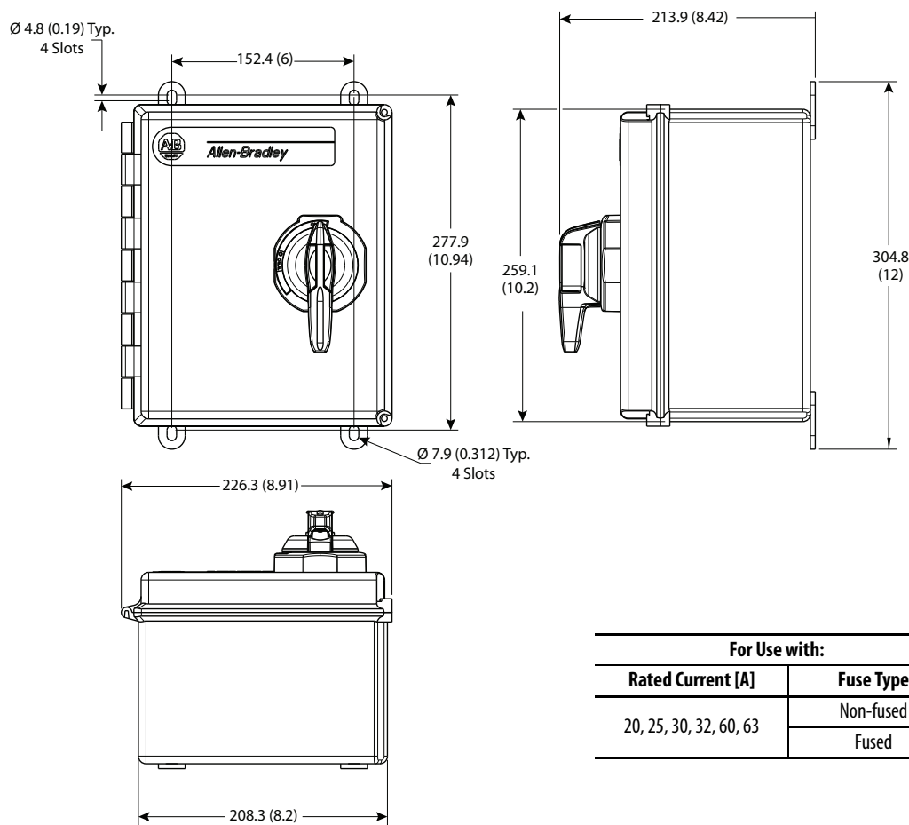
Figure 26 - IP66 (Type 3/4/4X/12) Corrosion-resistant, Non-metallic Enclosure
