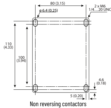
Figure 72 - Drilling Template for 80 A 4-Pole Contactors
